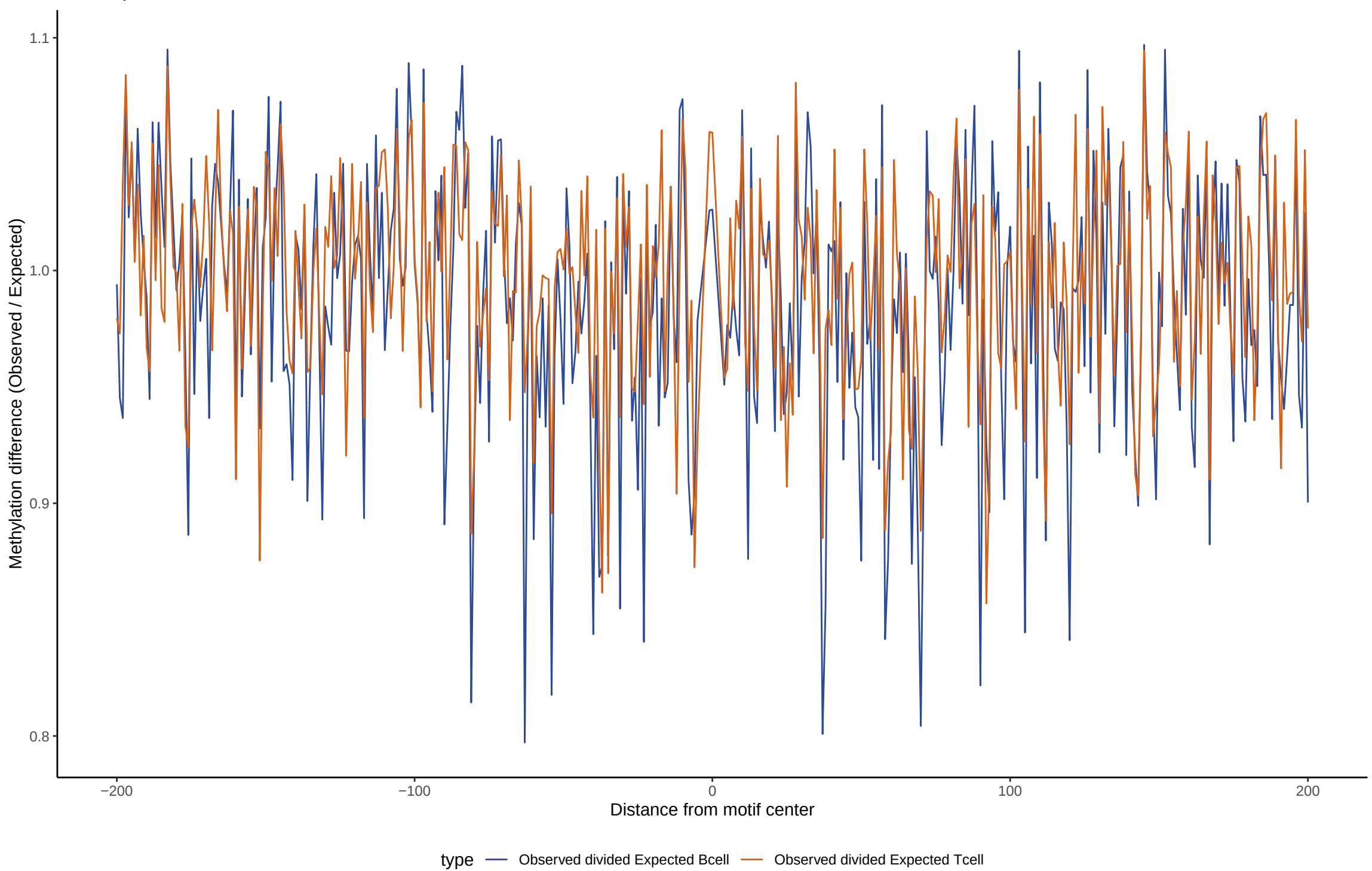
TF footprint difference for TEF
