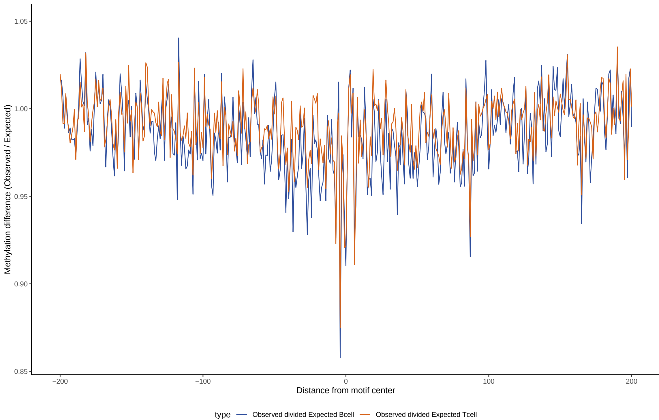
TF footprint difference for TFAP2A(var.2)
