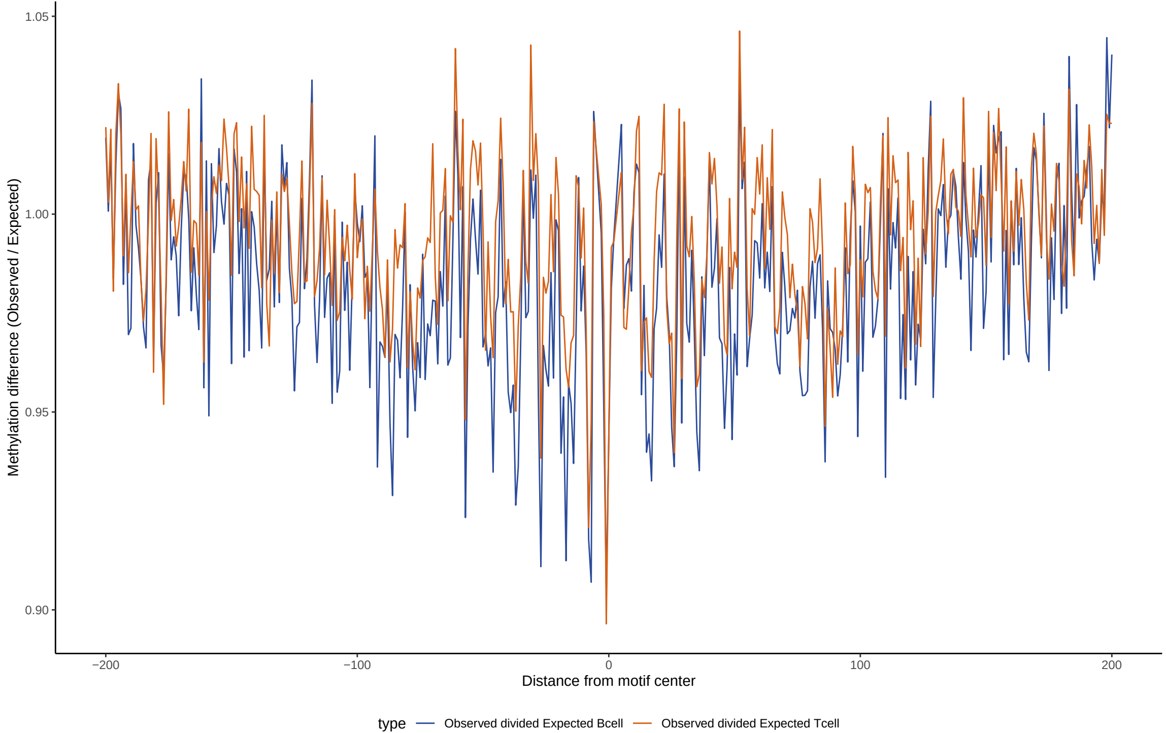
TF footprint difference for TFAP2B(var.3)
