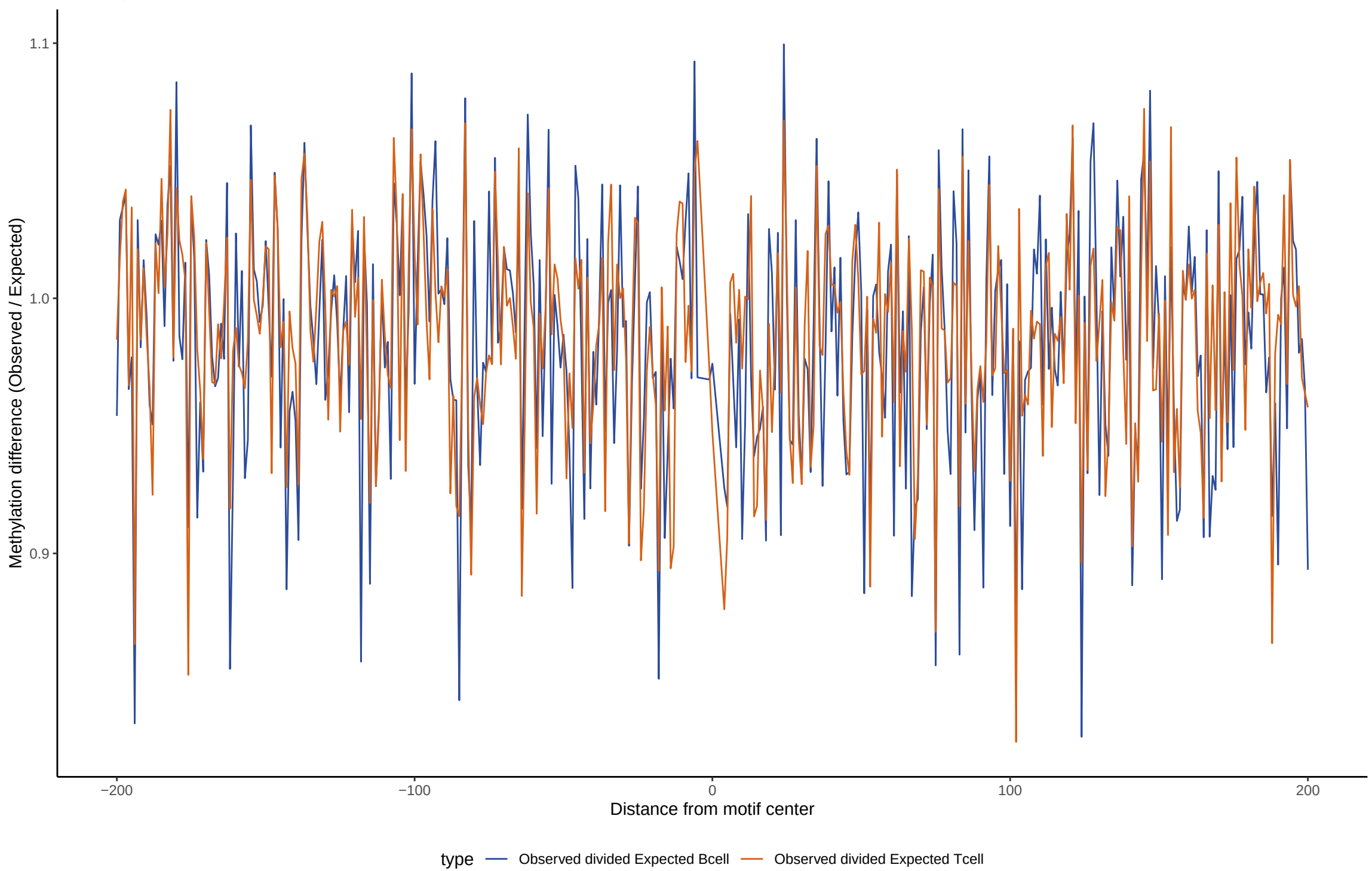
TF footprint difference for TFCP2
