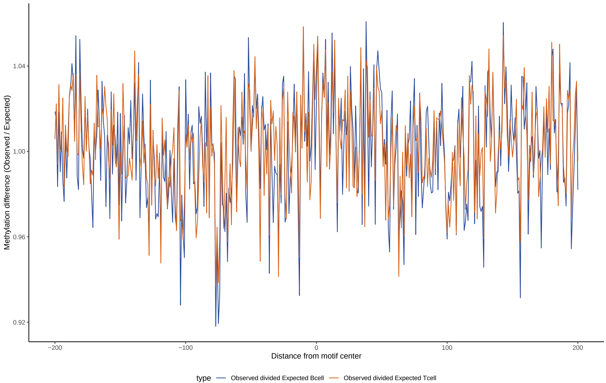
TF footprint difference for TFDP1
