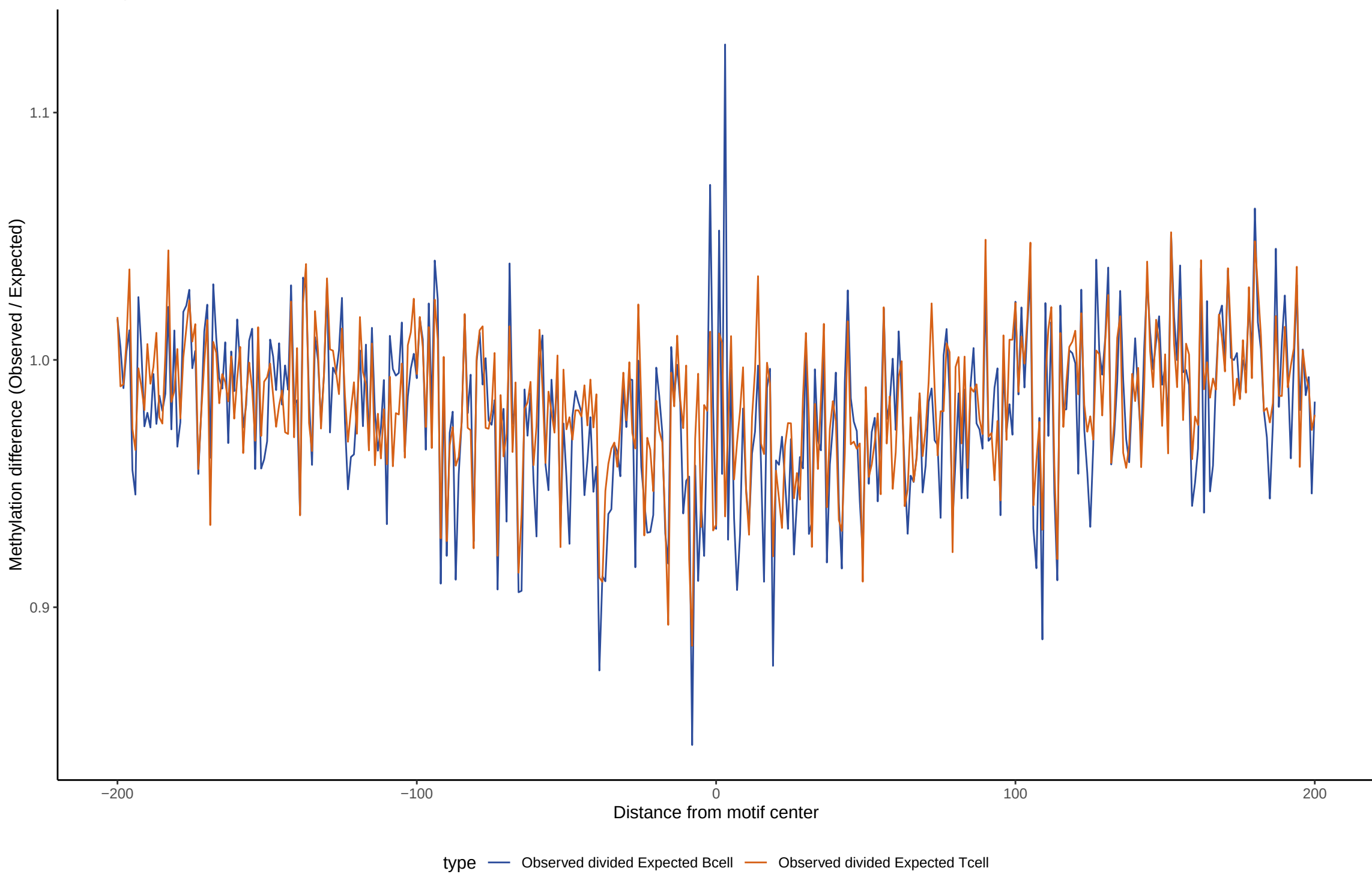
TF footprint difference for TGIF2
