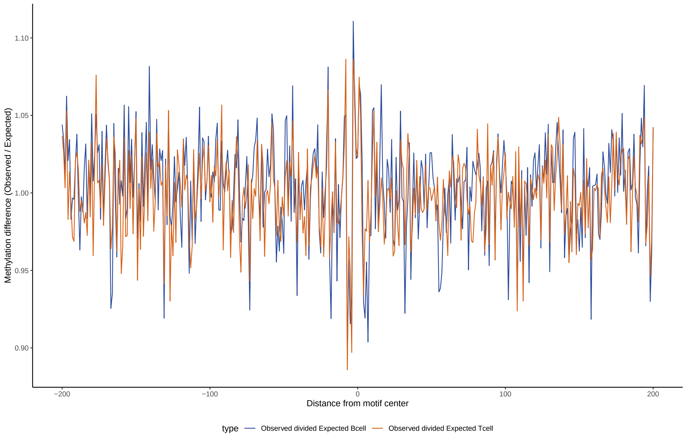
TF footprint difference for TP53
