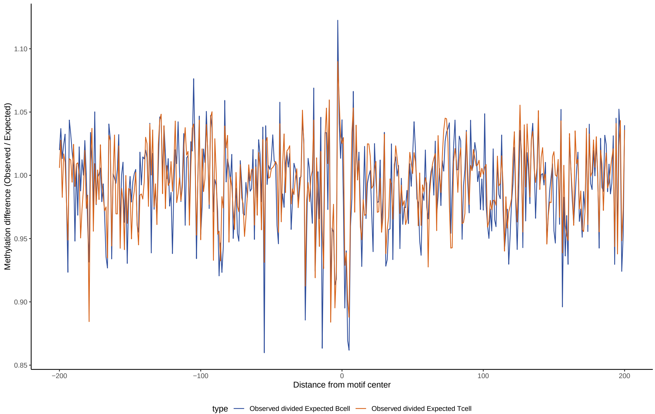
TF footprint difference for TP63
