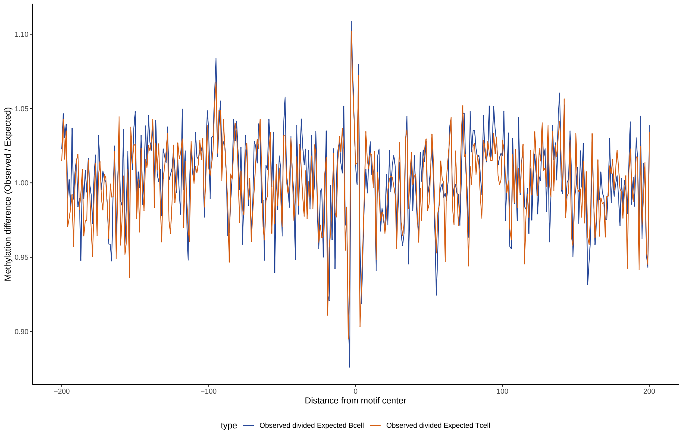
TF footprint difference for TP73
