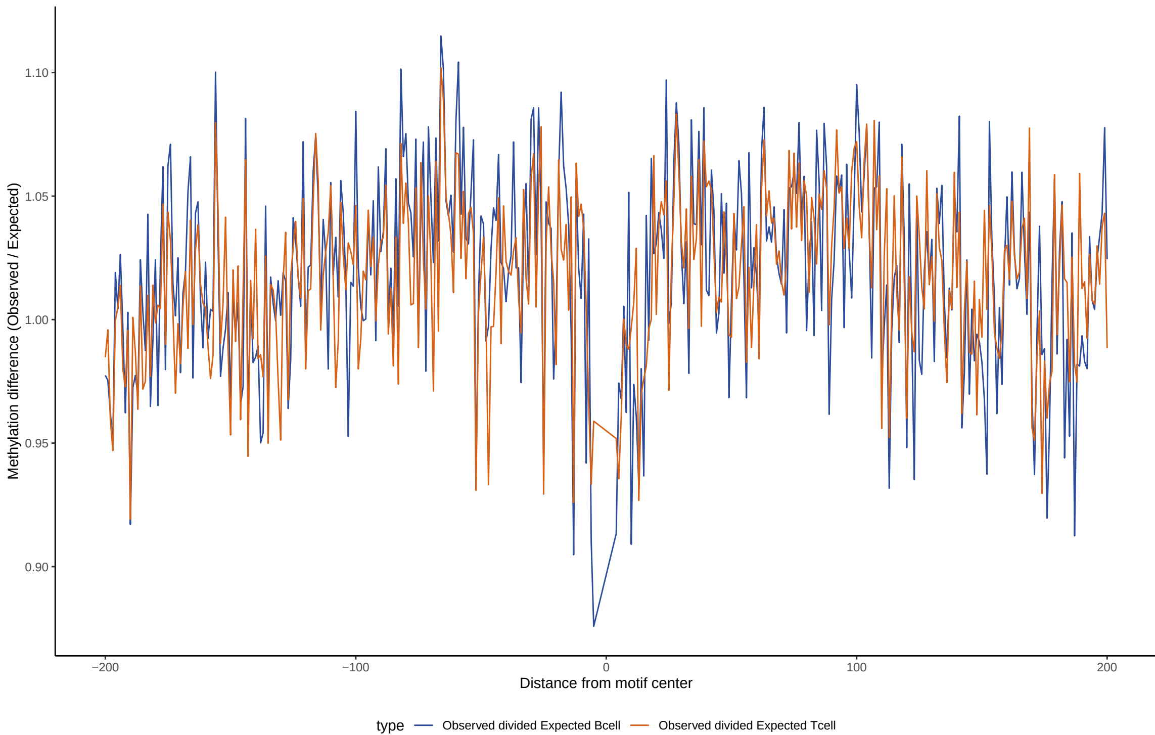
TF footprint difference for UNCX
