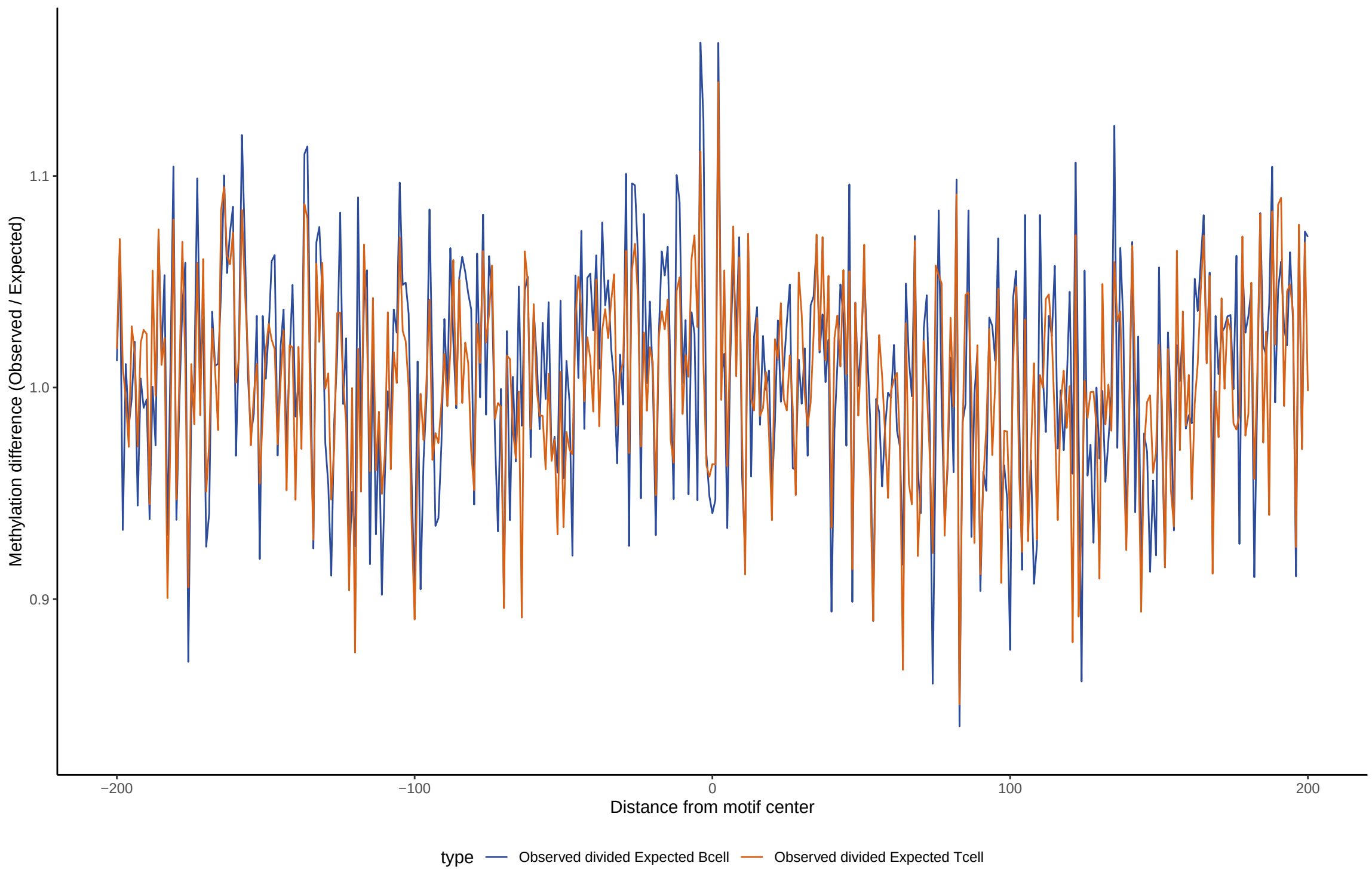
TF footprint difference for XBP1
