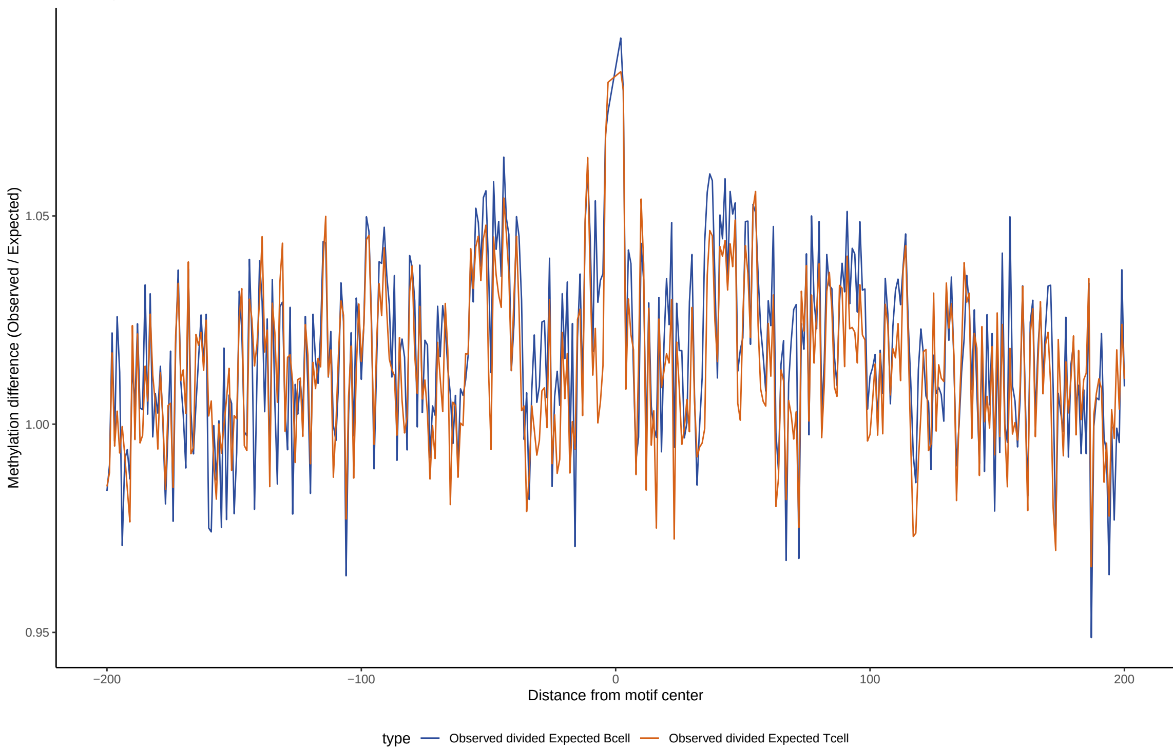
TF footprint difference for YY1
