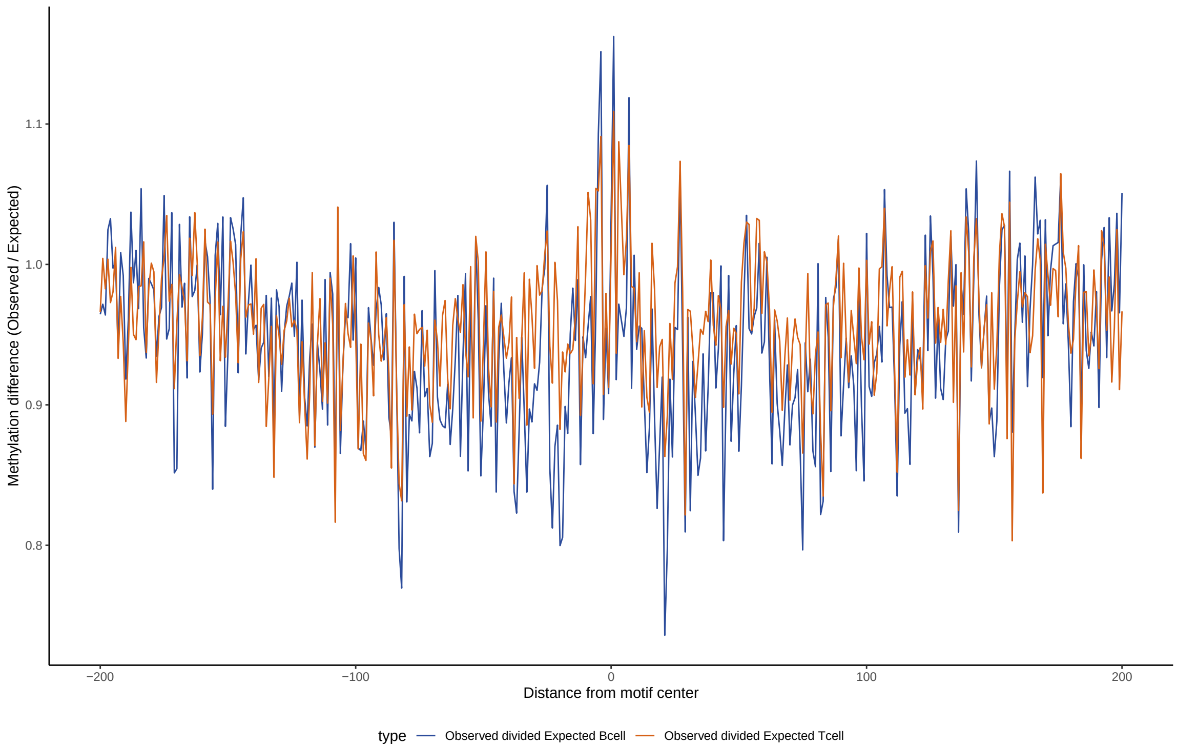
TF footprint difference for ZBTB33
