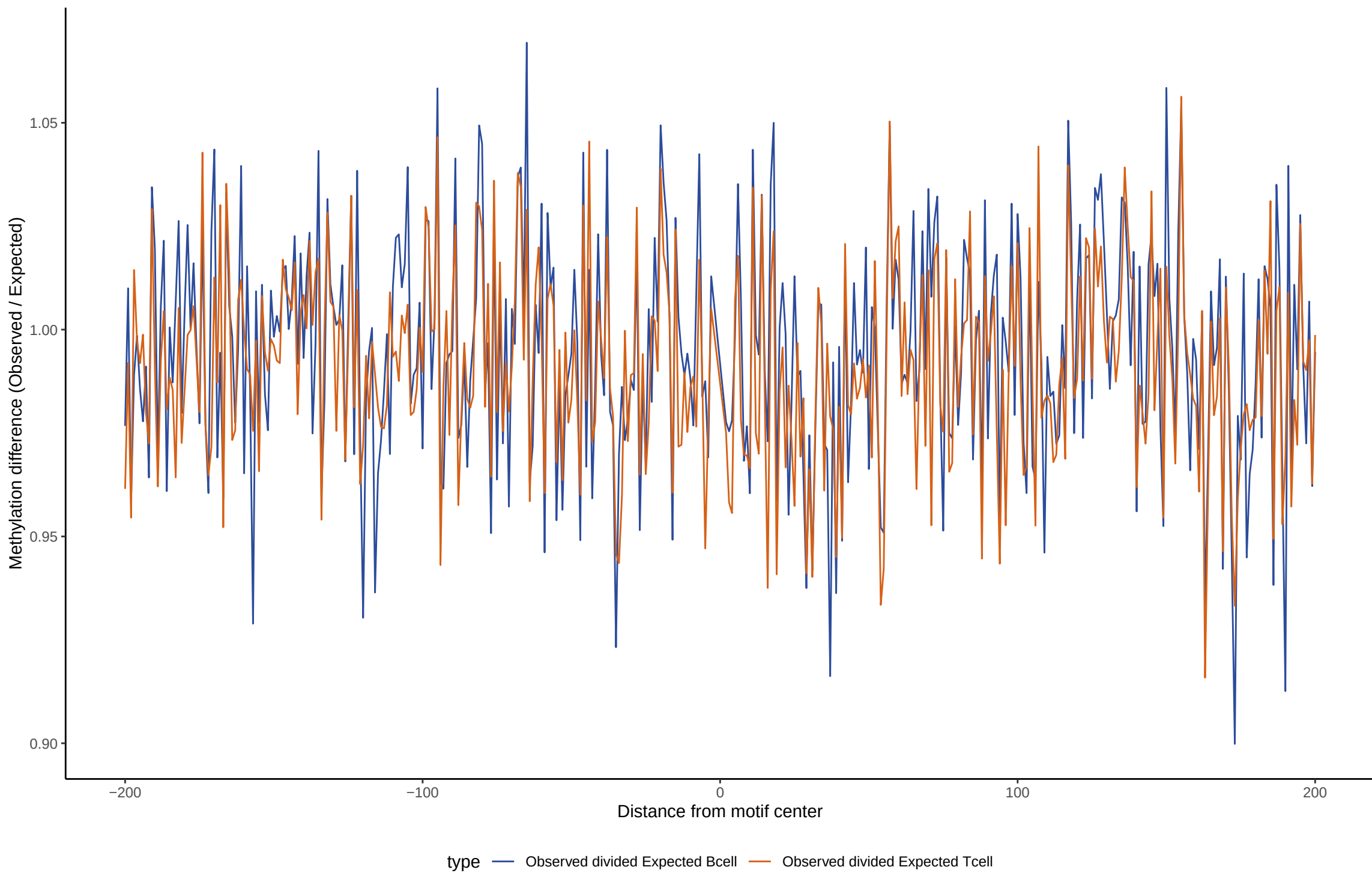
TF footprint difference for ZBTB7B
