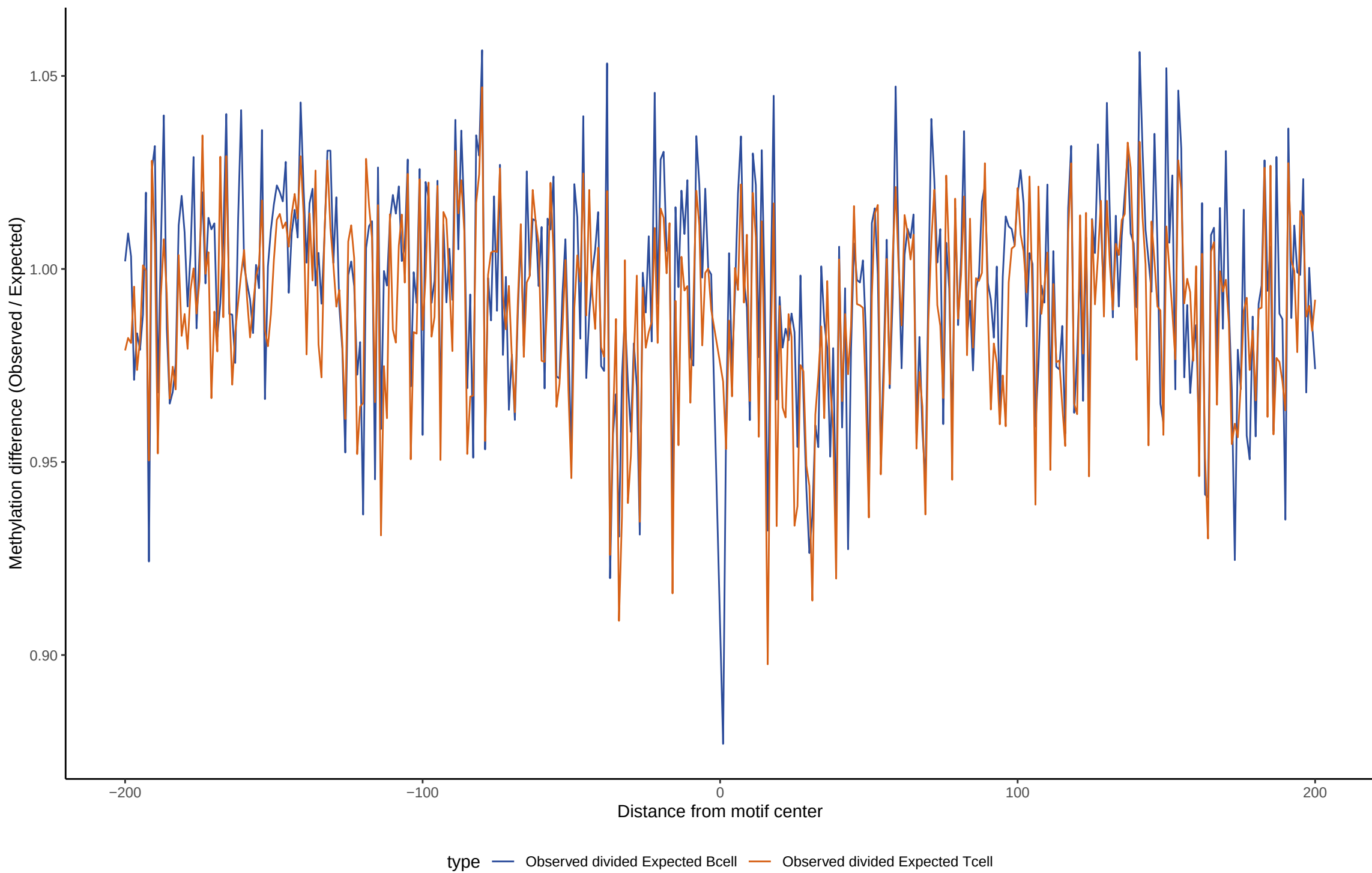
TF footprint difference for ZBTB7C
