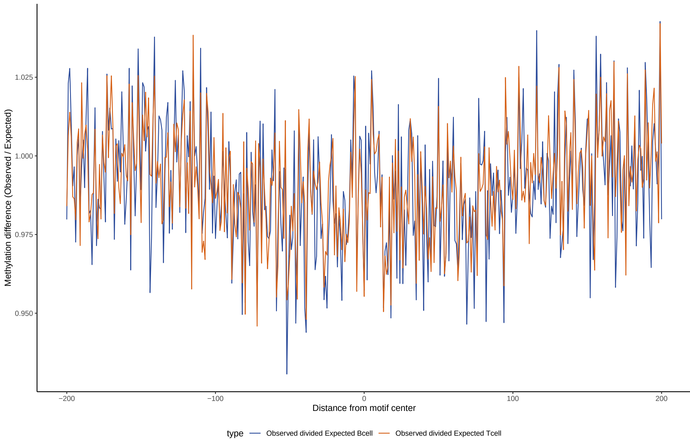
TF footprint difference for ZIC1
