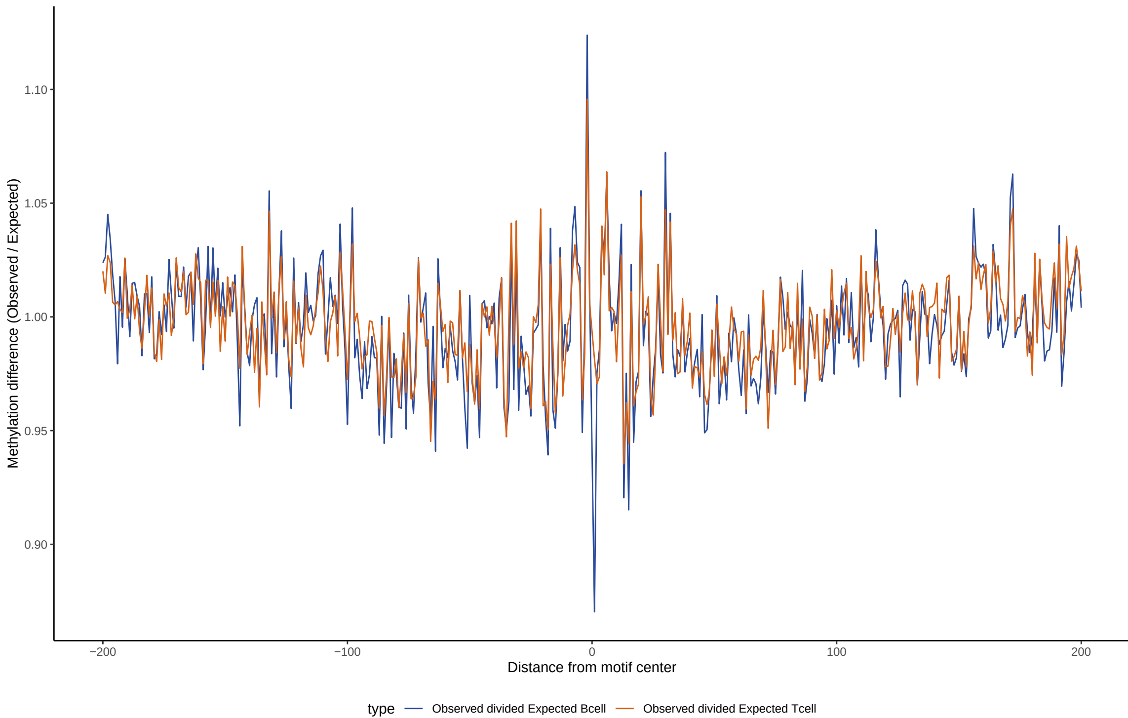
TF footprint difference for ZIC3
