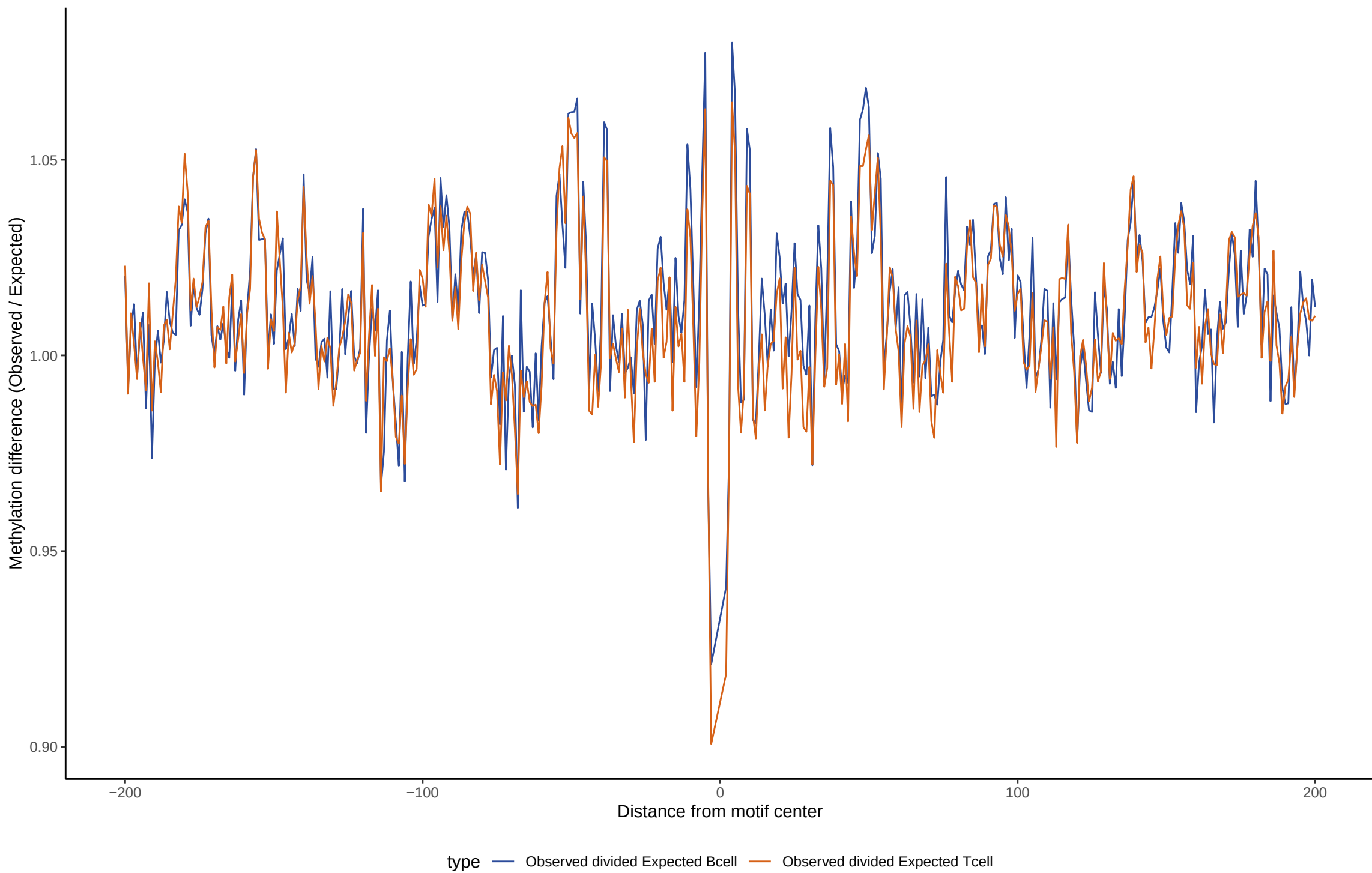
TF footprint difference for ZNF354C
