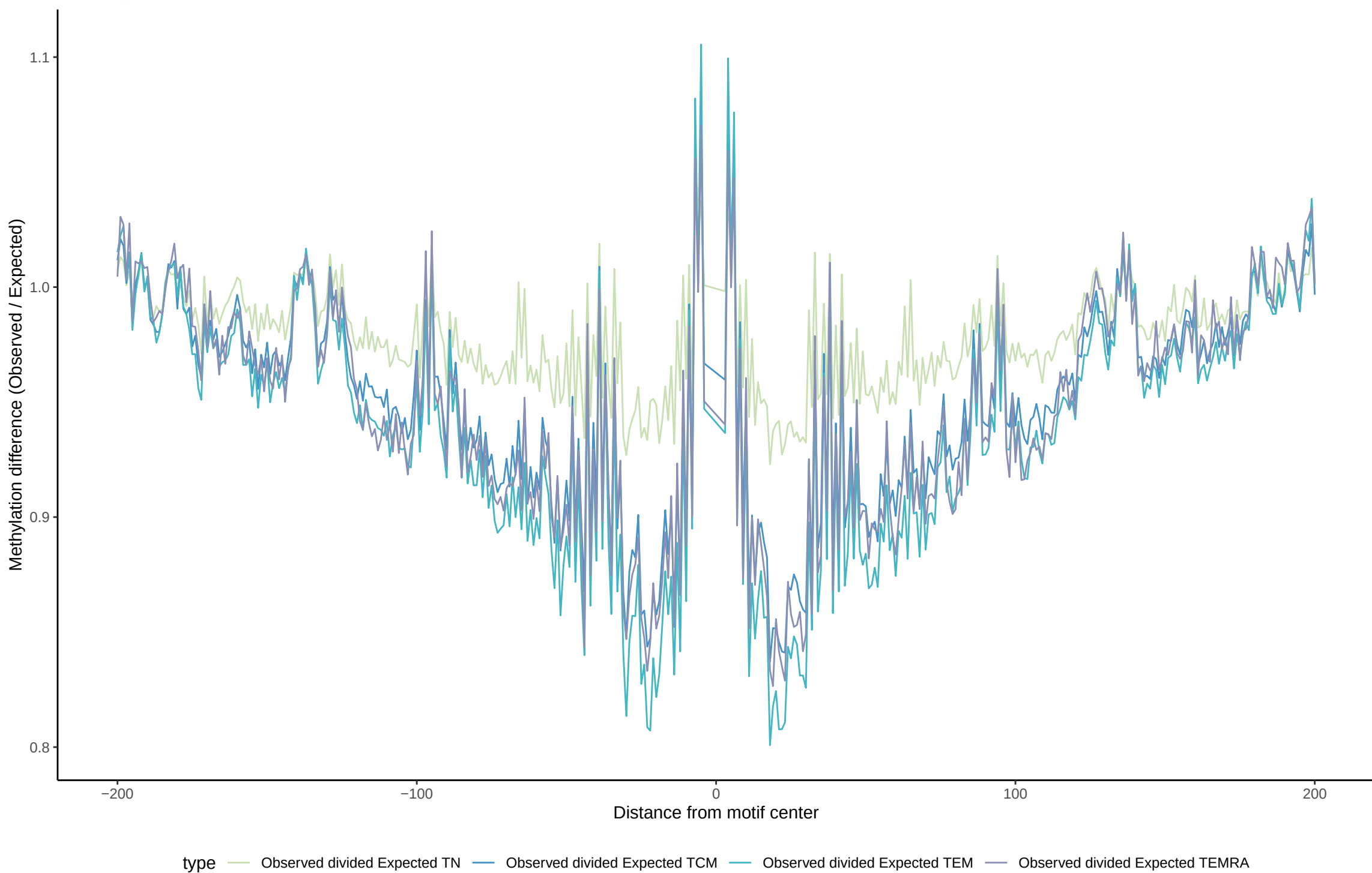
TF footprint difference for FOSL2
