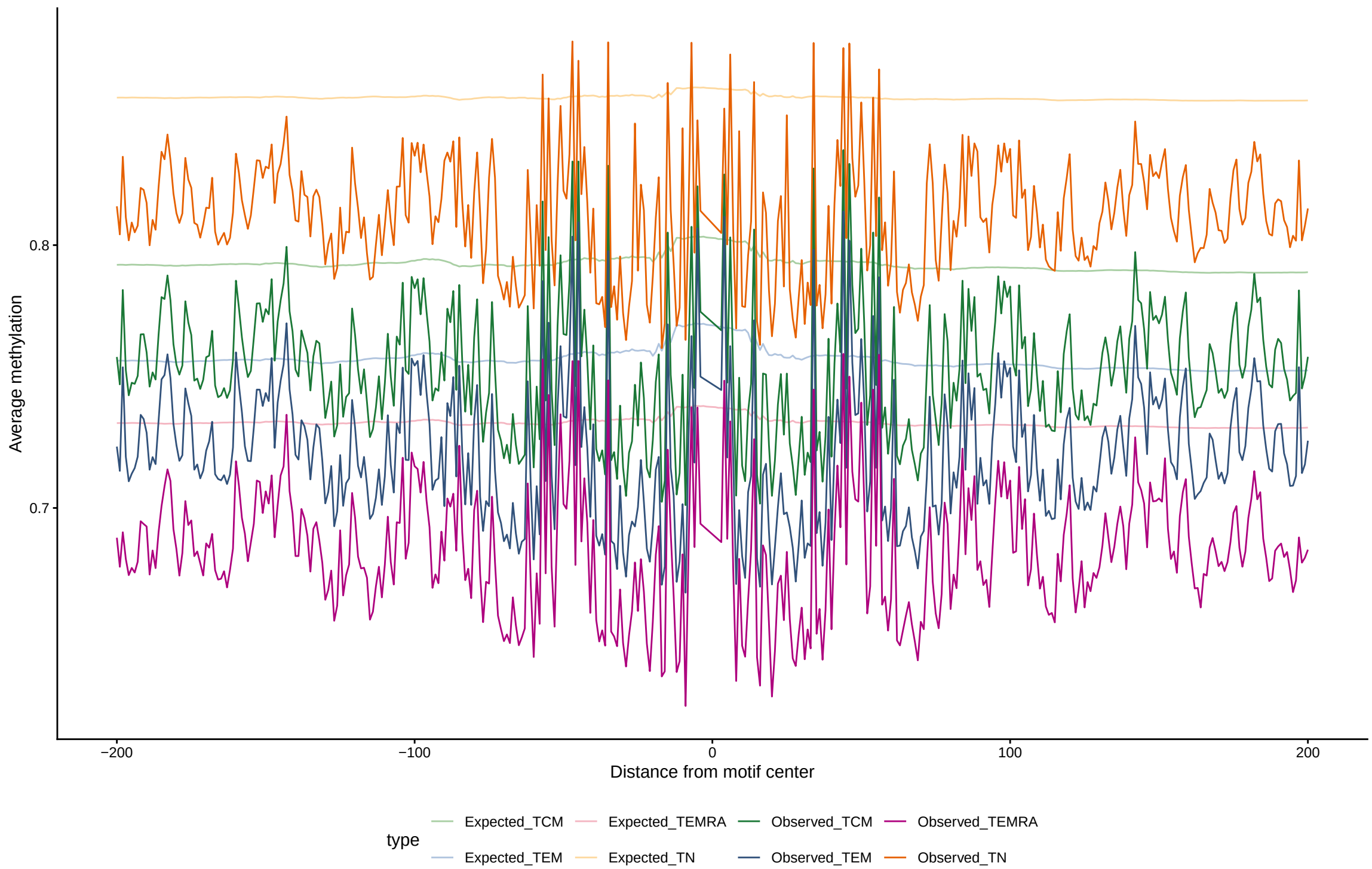
Expected vs observed footprints for ASCL1(var.2)
