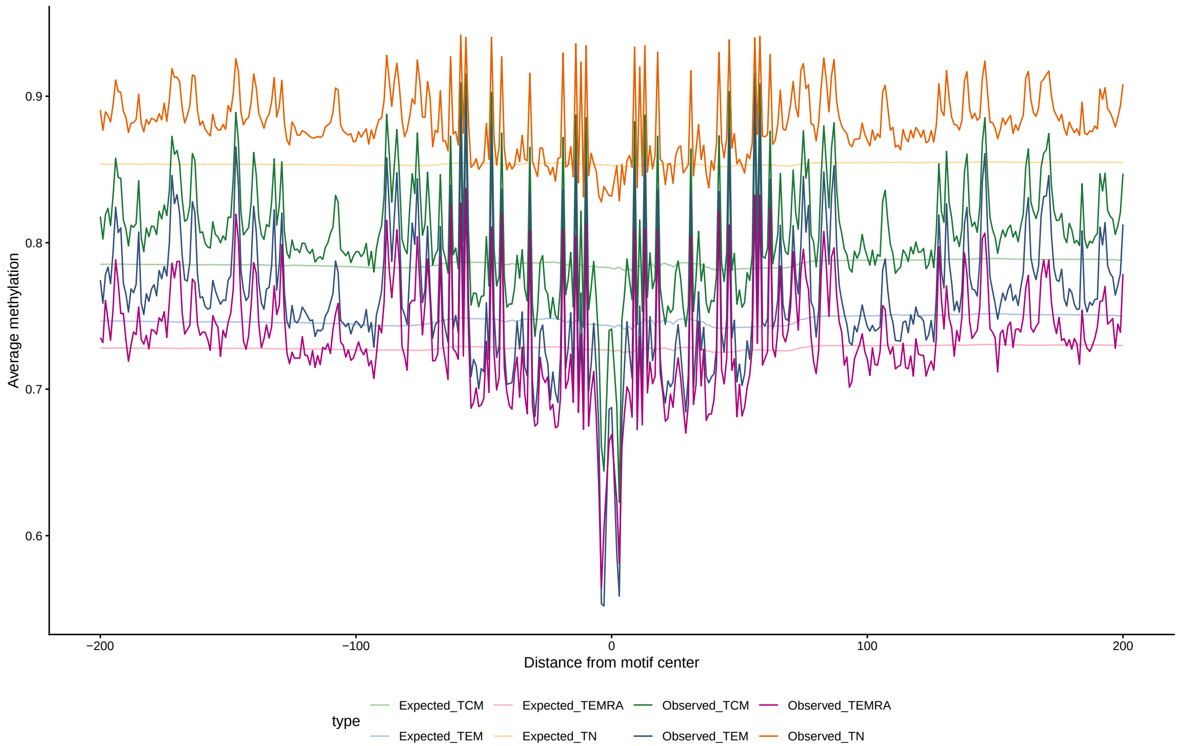
Expected vs observed footprints for ATF2
