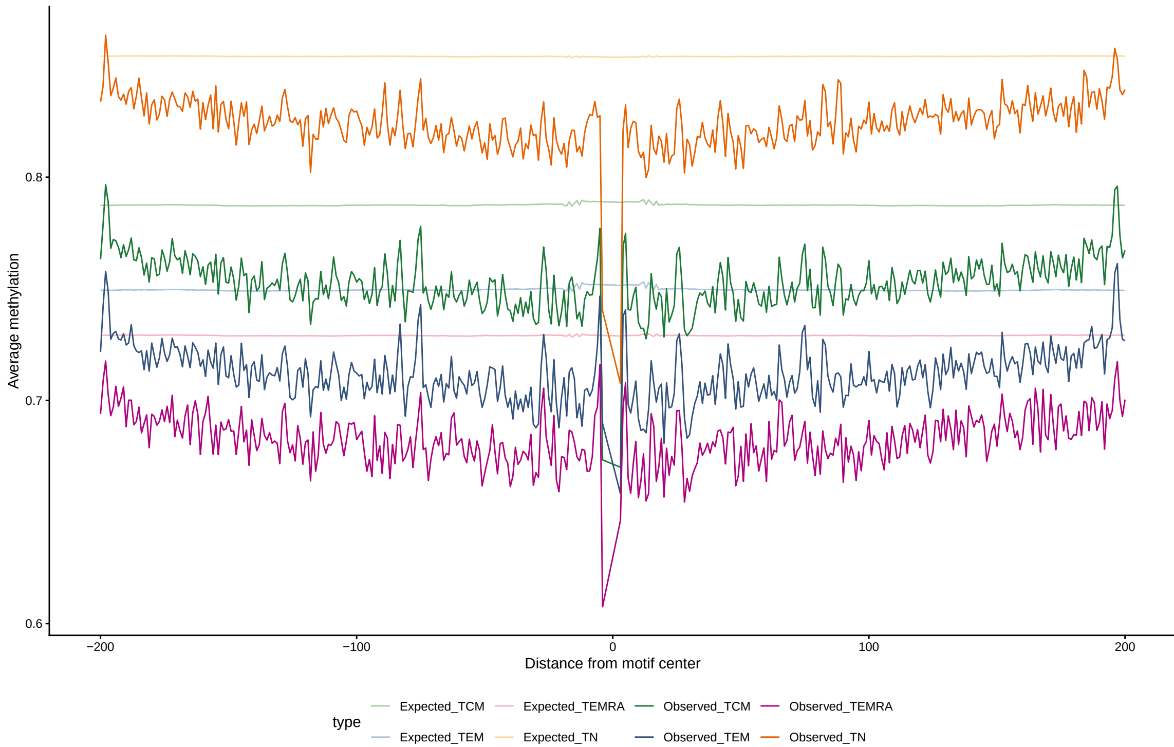
Expected vs observed footprints for ATOH1(var.2)
