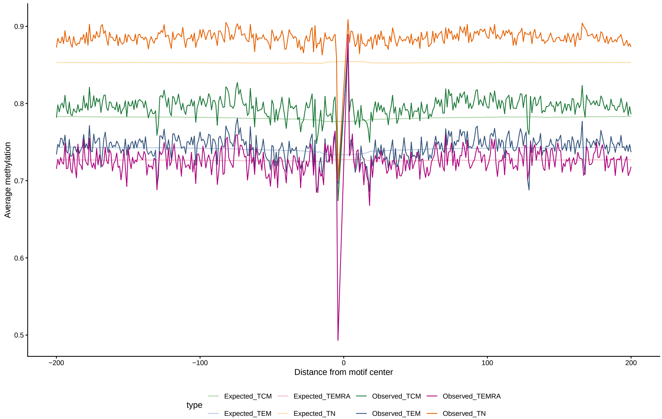
Expected vs observed footprints for BARX1
