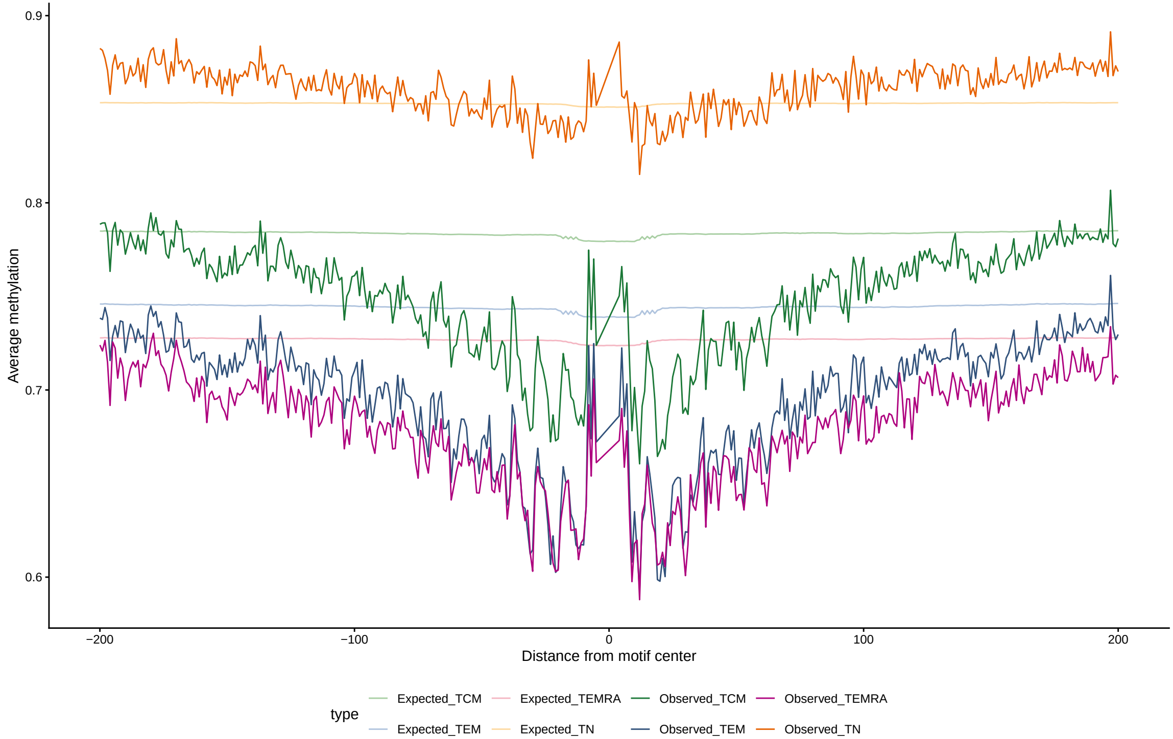
Expected vs observed footprints for BATF::JUN
