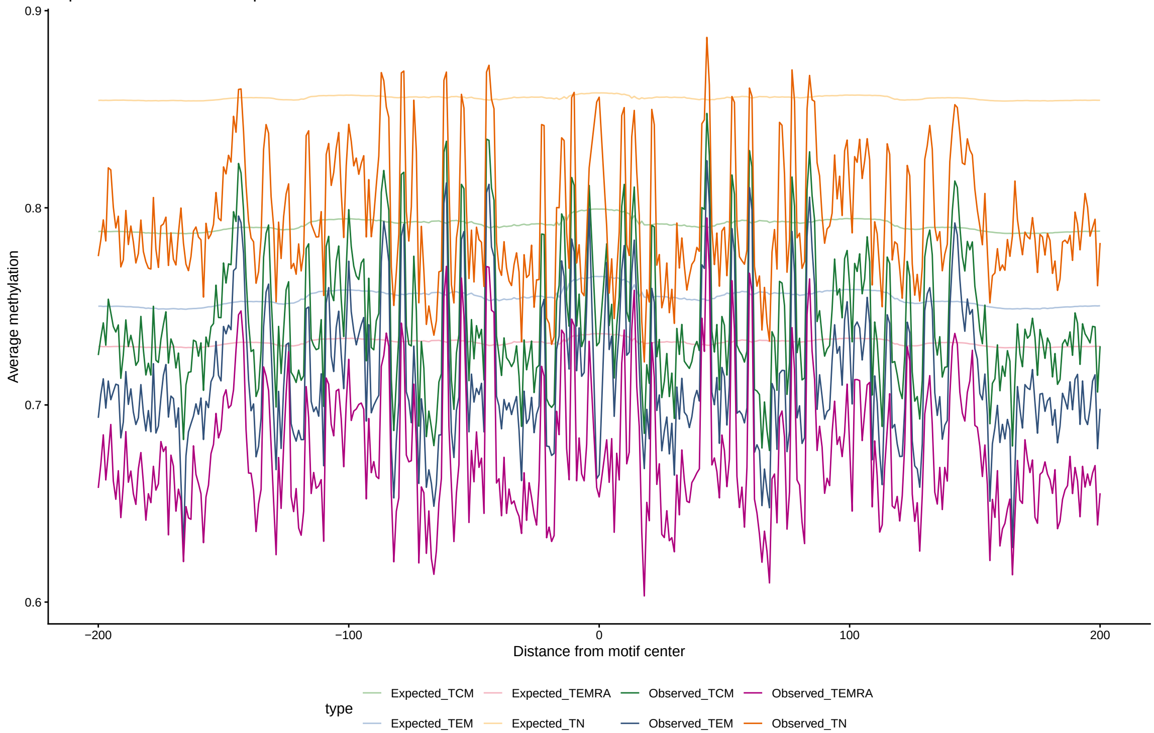
Expected vs observed footprints for BHLHE40
