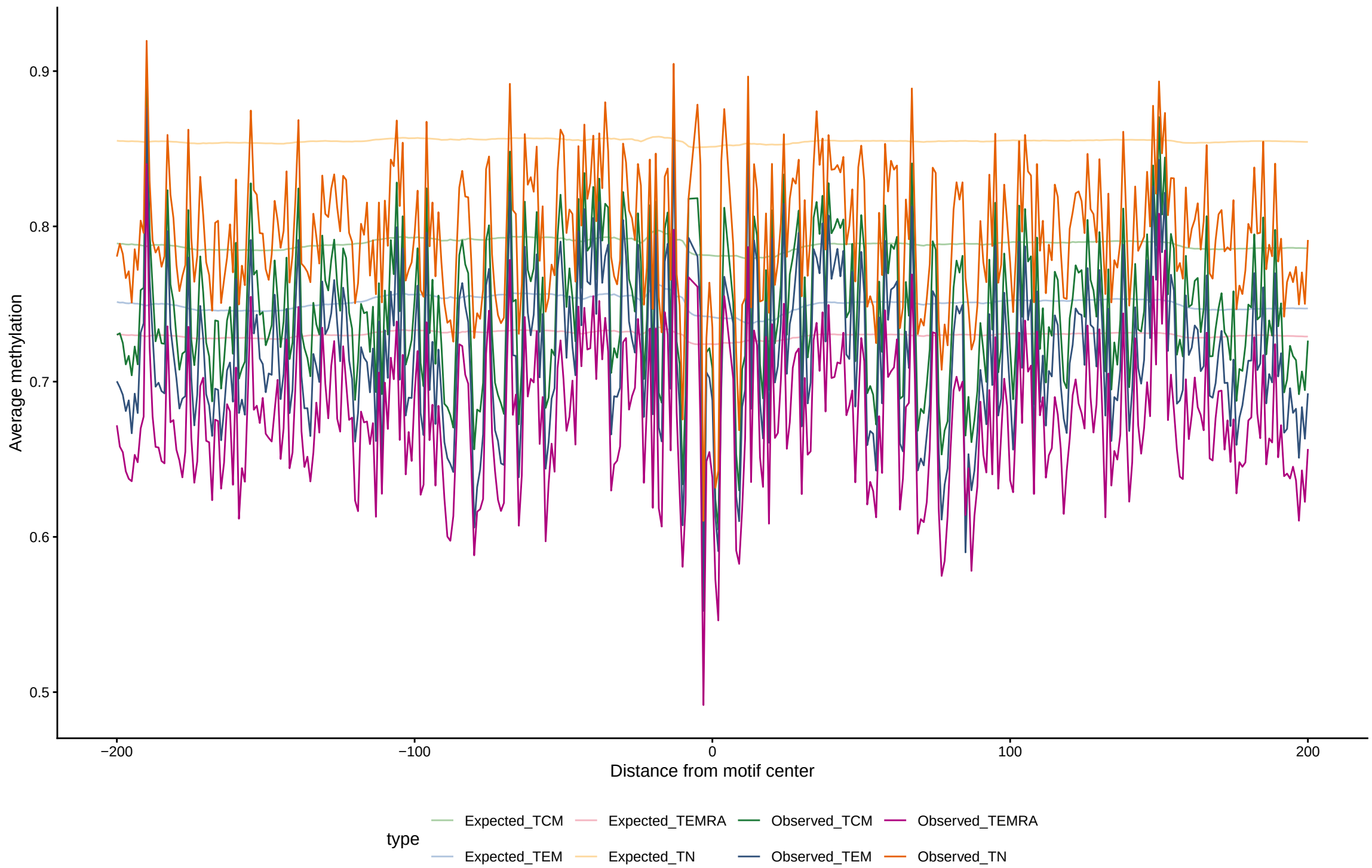
Expected vs observed footprints for CENPB
