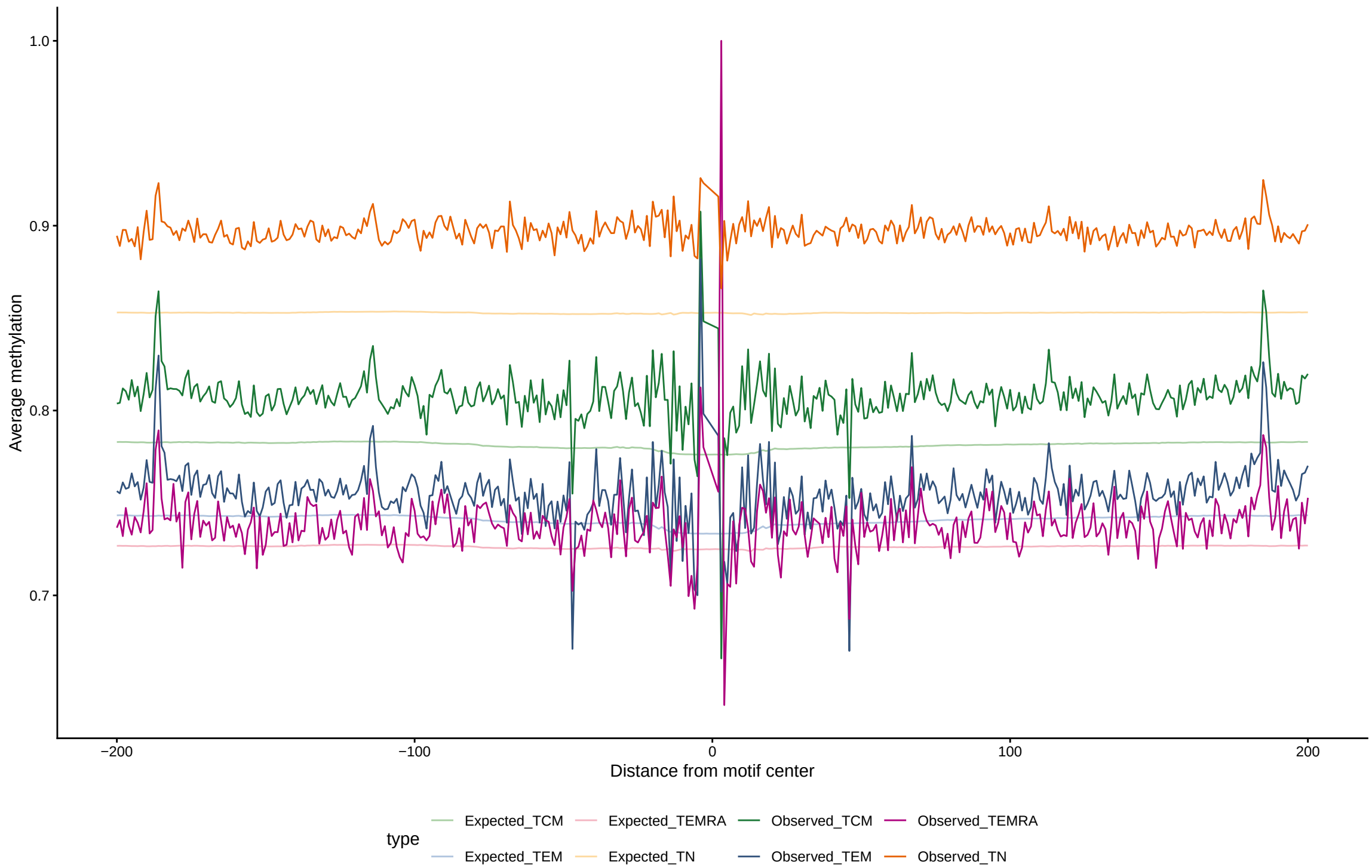
Expected vs observed footprints for DMRT3
