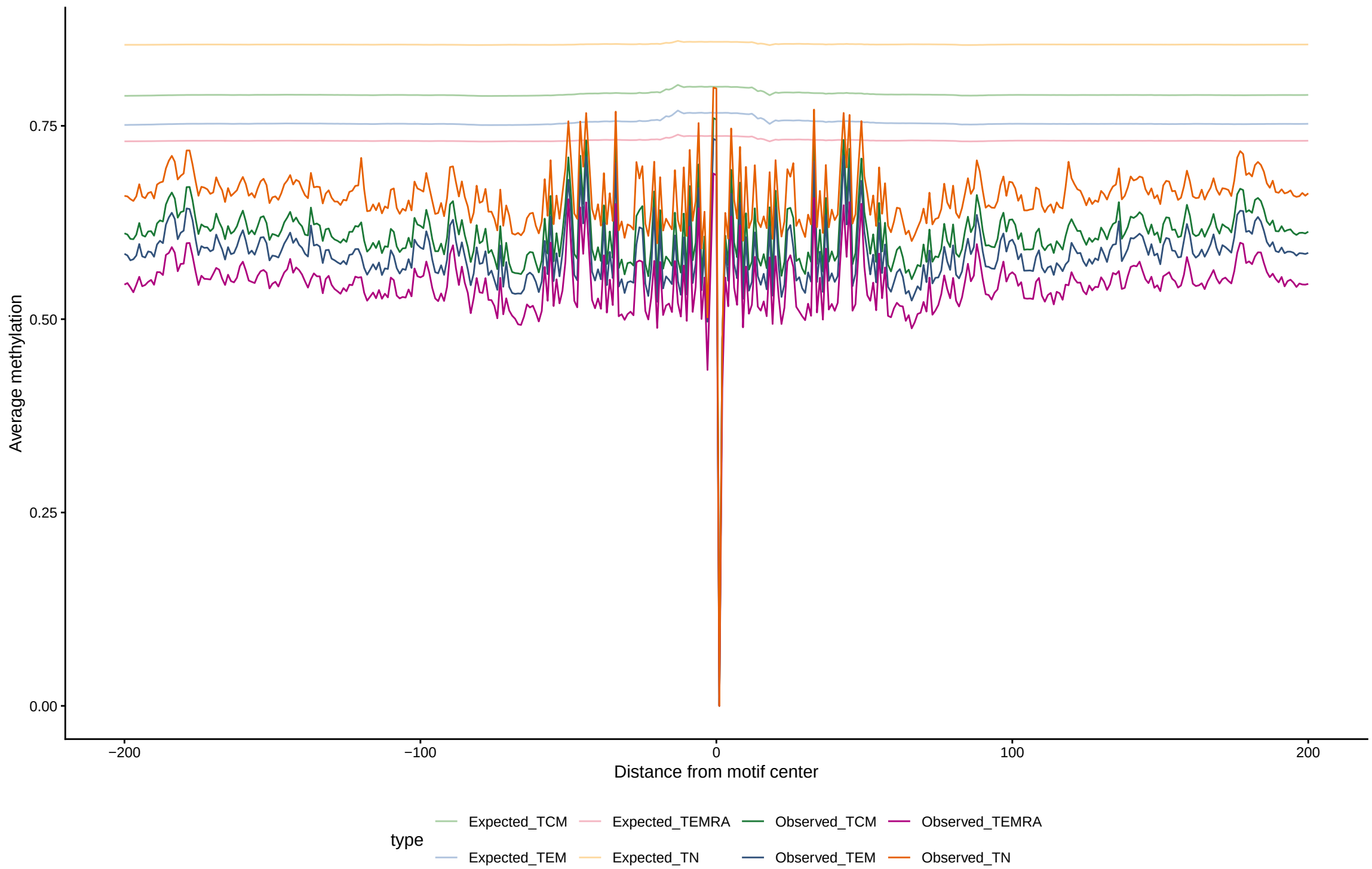
Expected vs observed footprints for E2F6
