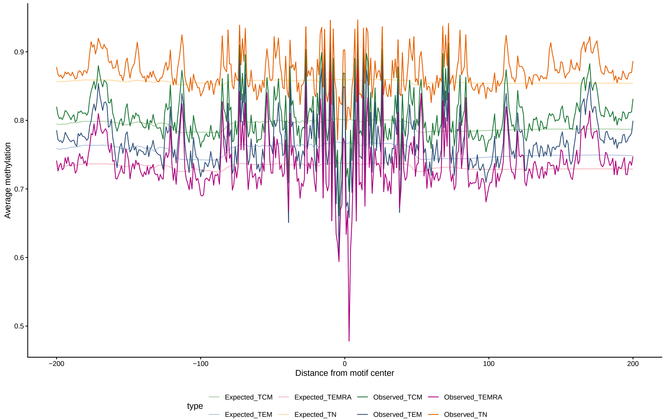
Expected vs observed footprints for ESR1
