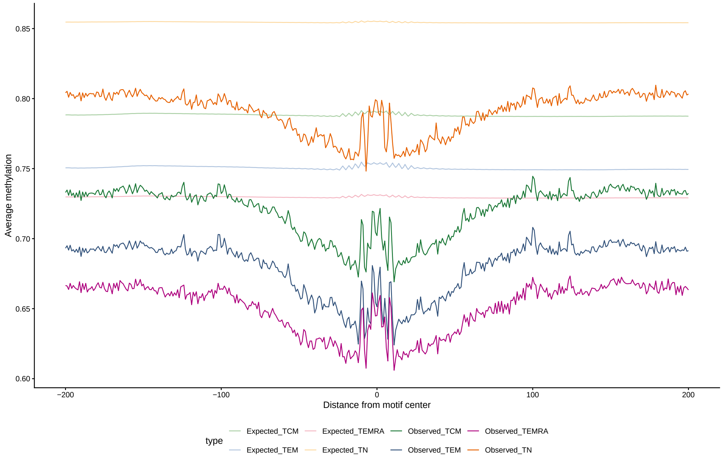
Expected vs observed footprints for EWSR1-FLI1
