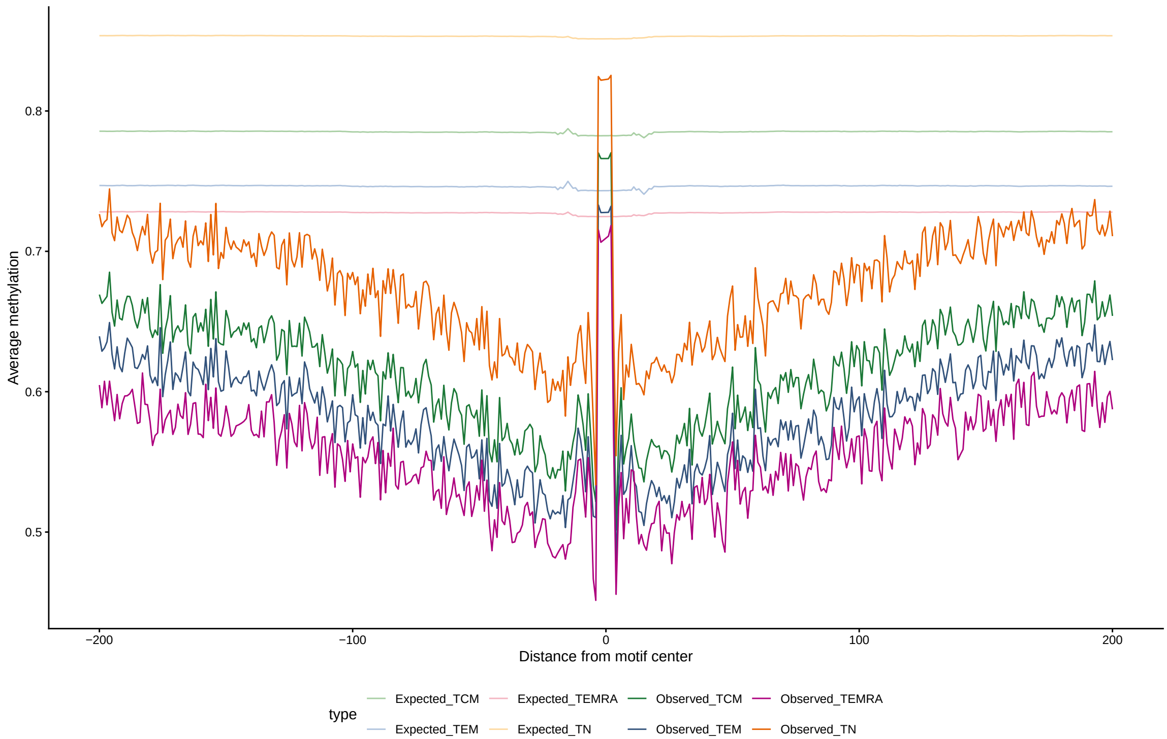
Expected vs observed footprints for FLI1
