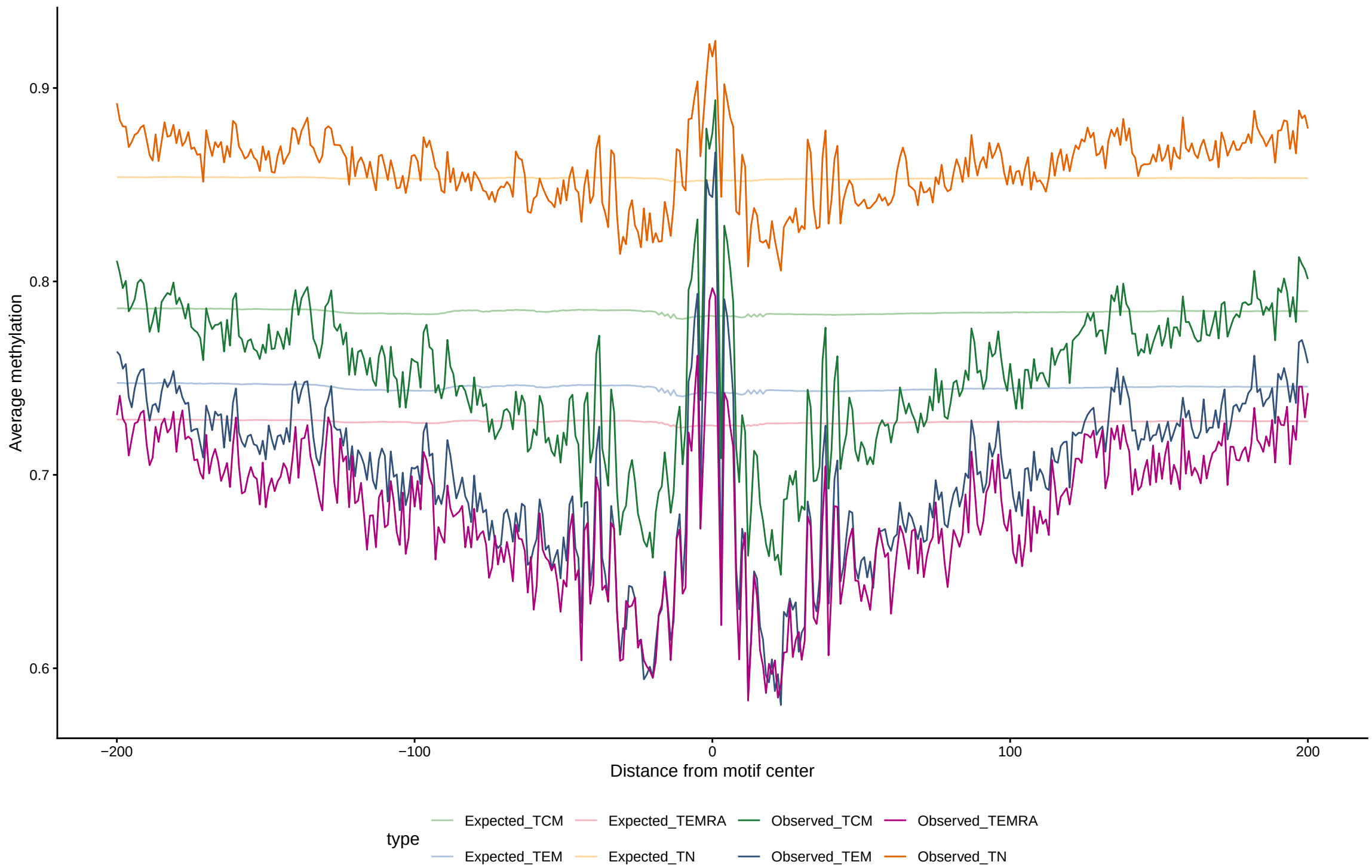
Expected vs observed footprints for FOS::JUN
