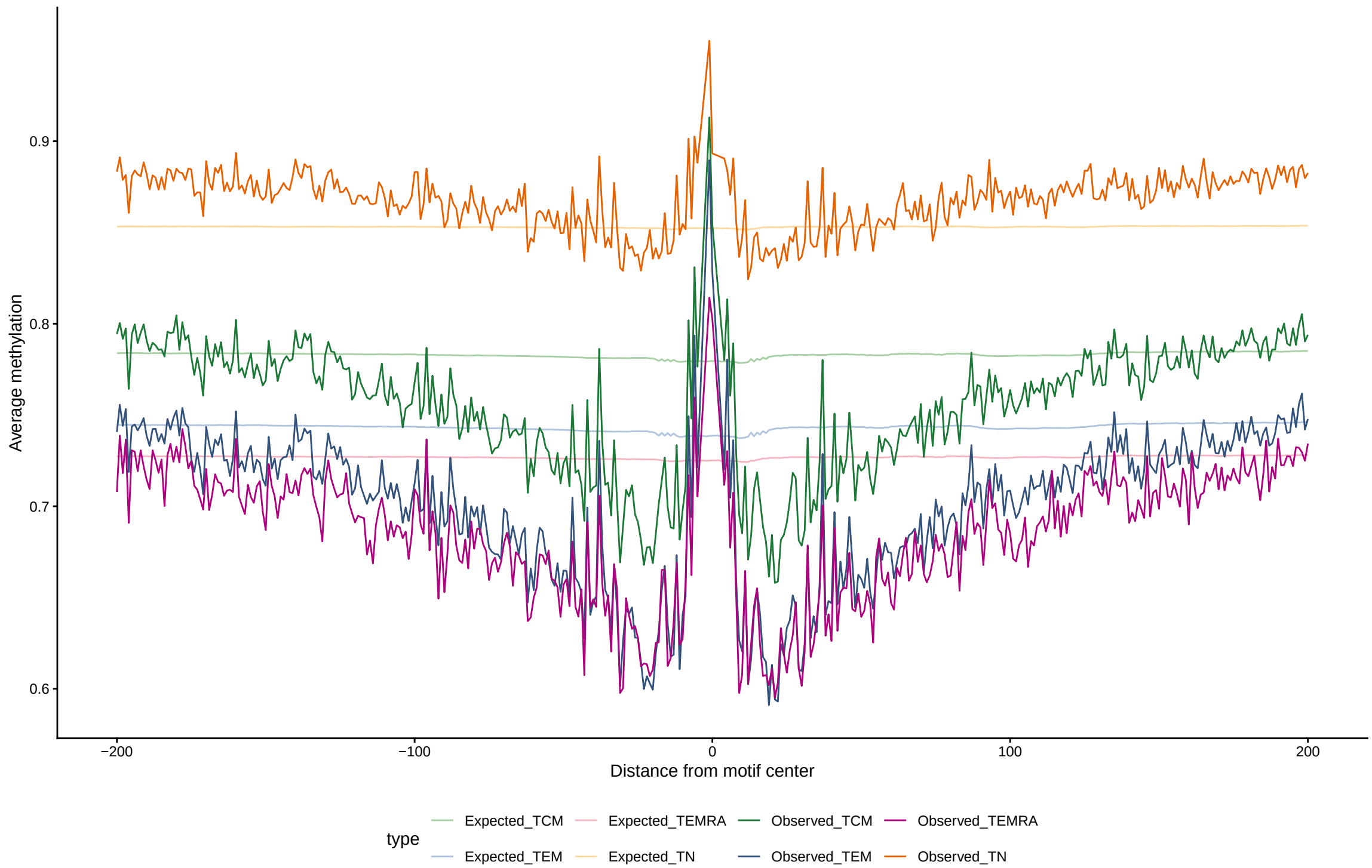
Expected vs observed footprints for FOSL1::JUNB
