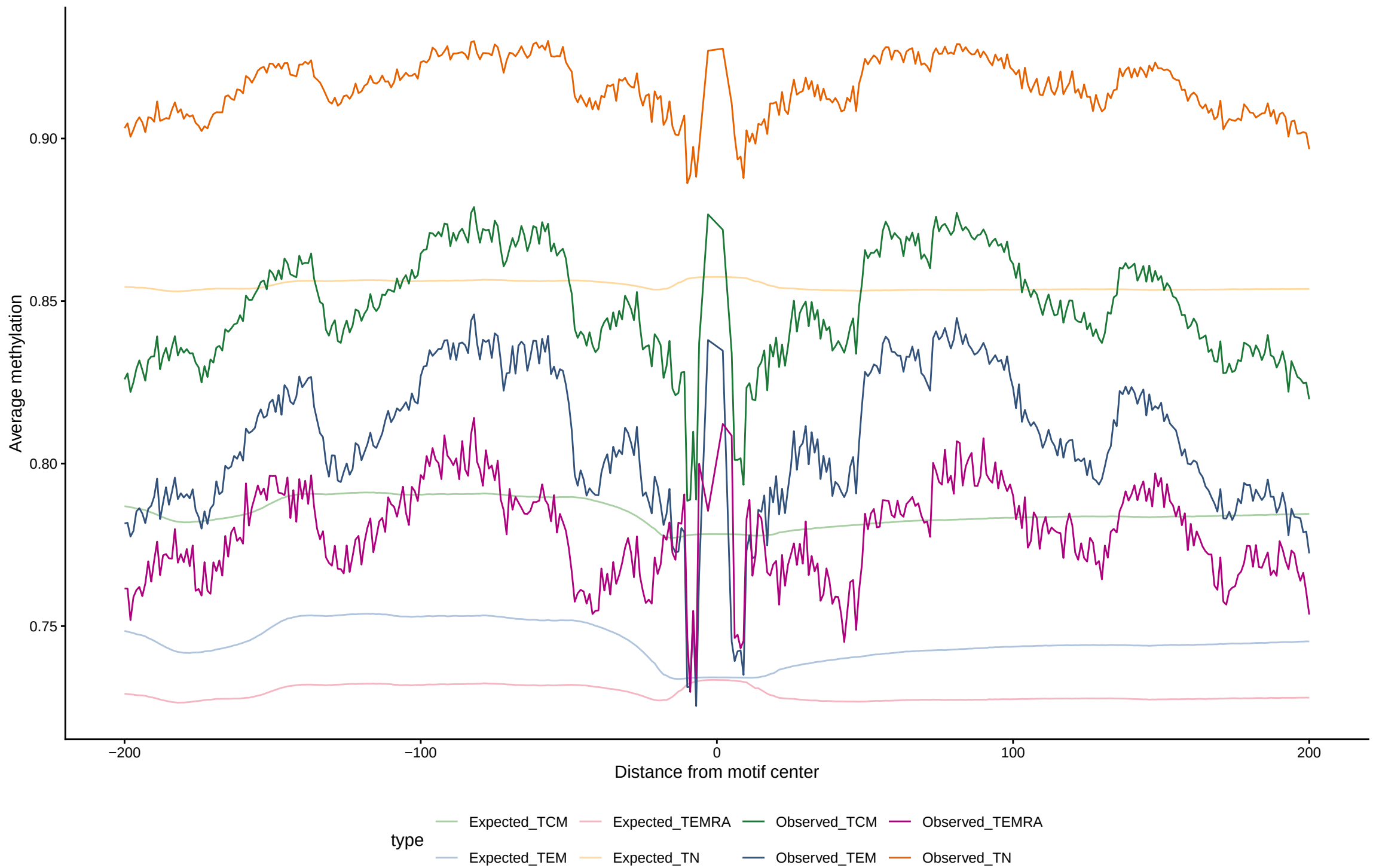
Expected vs observed footprints for FOXC1
