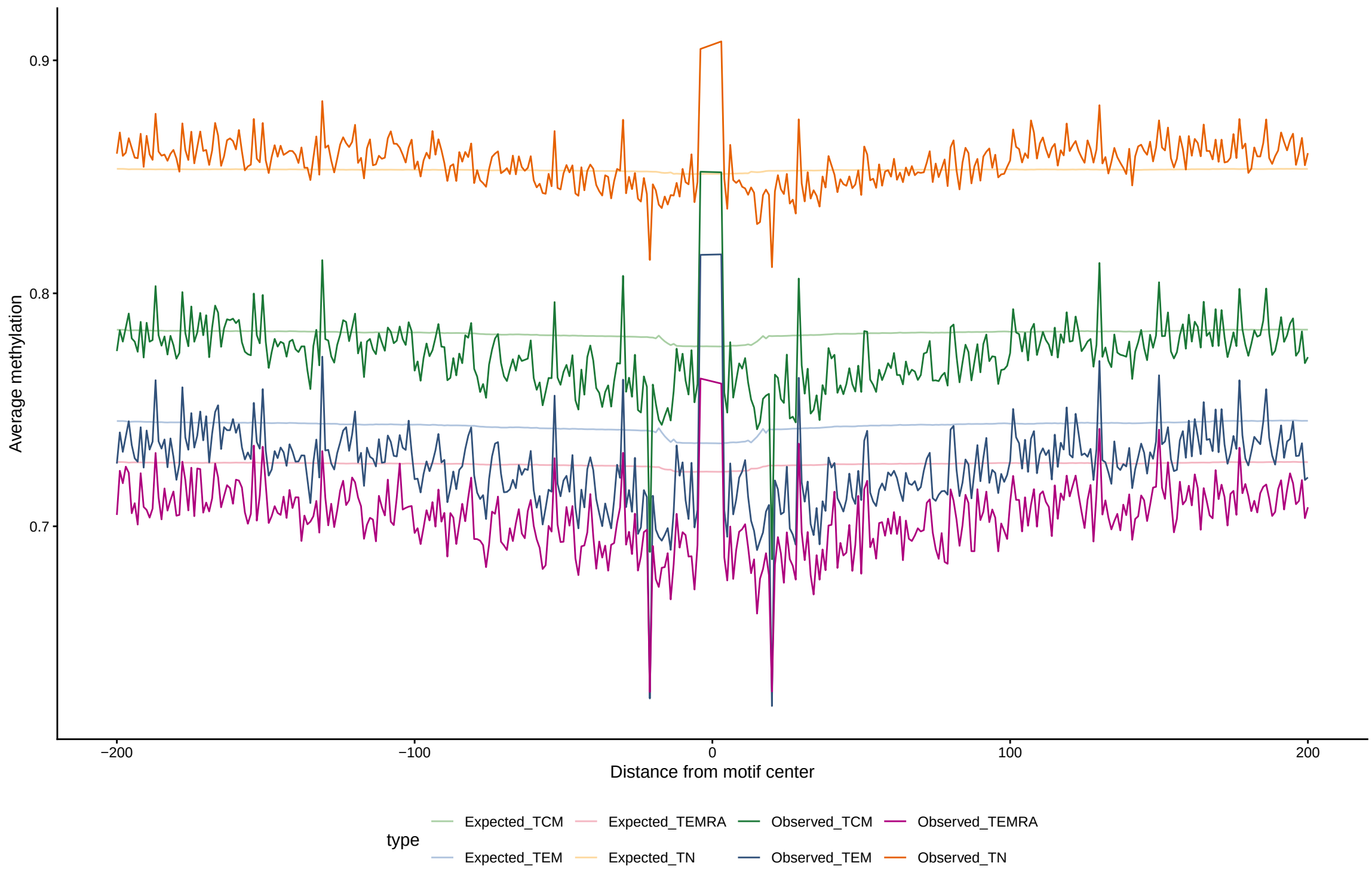
Expected vs observed footprints for FOXI1
