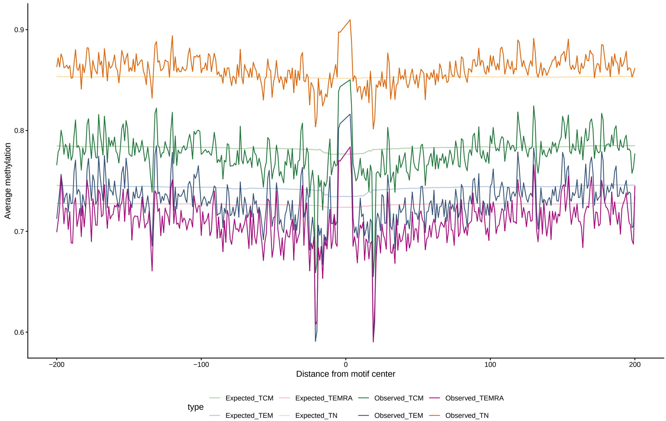
Expected vs observed footprints for FOXO3
