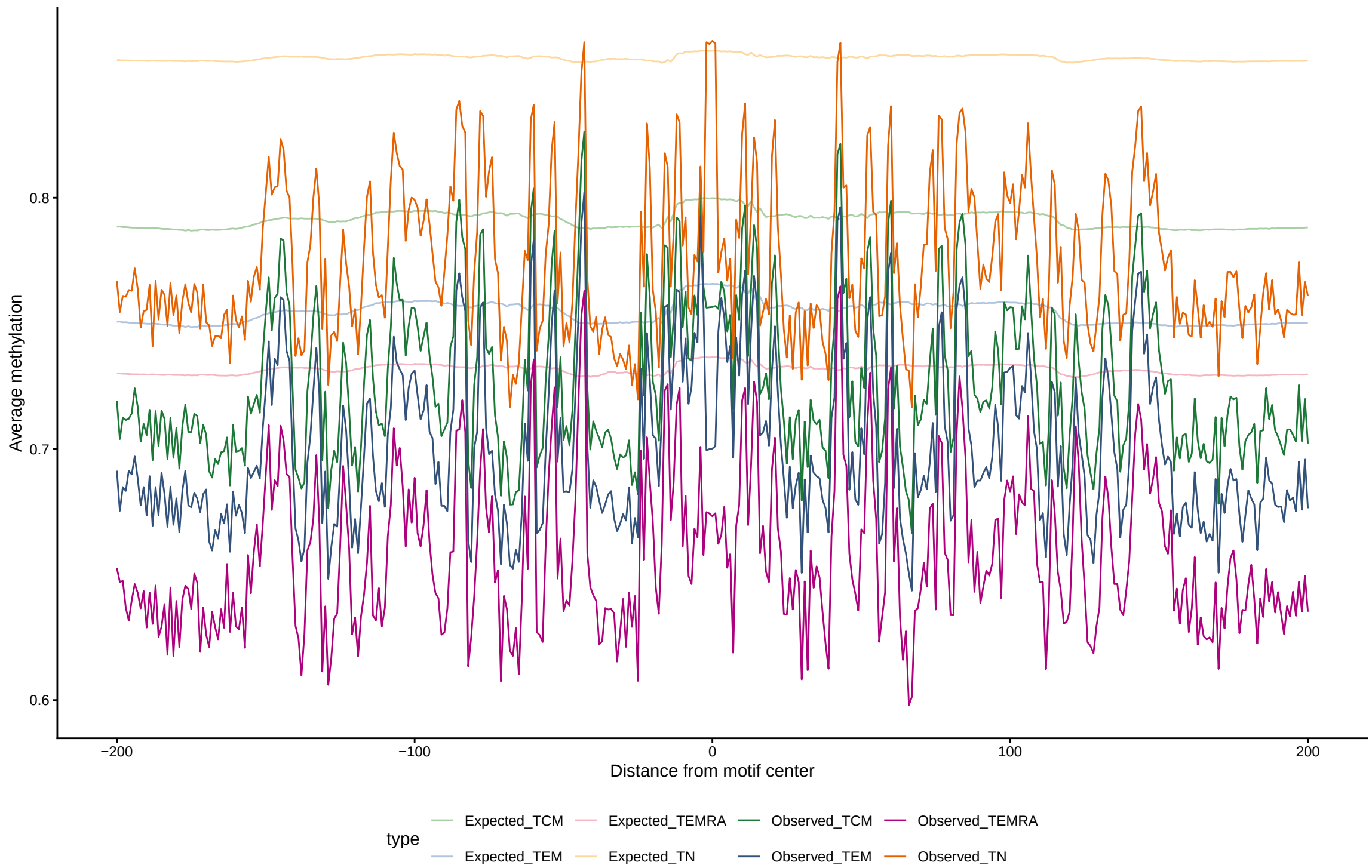
Expected vs observed footprints for HIF1A
