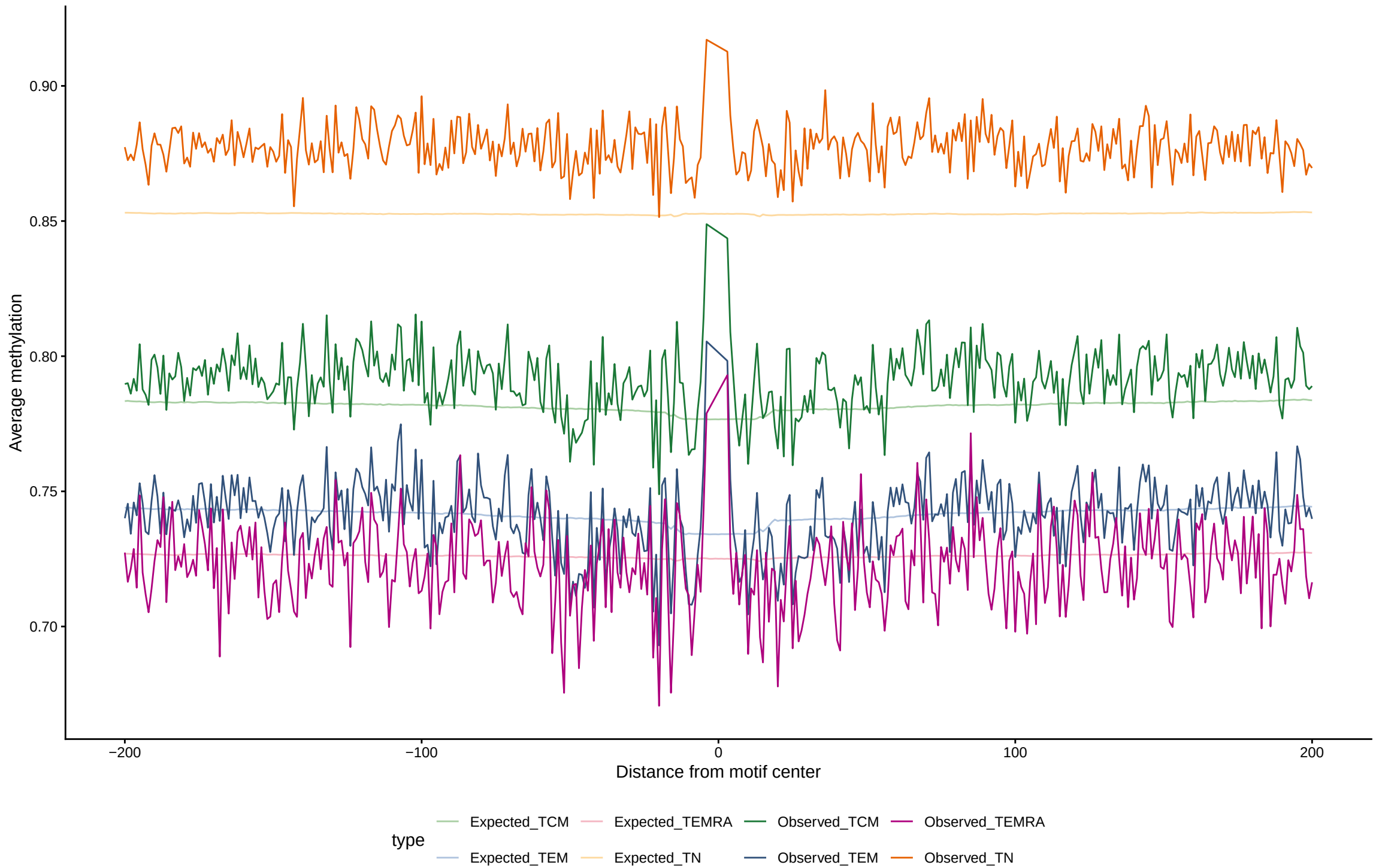
Expected vs observed footprints for HMBOX1
