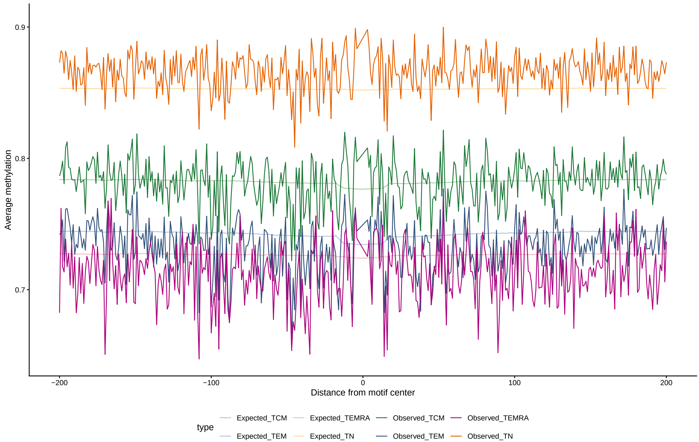
Expected vs observed footprints for HOXA1
