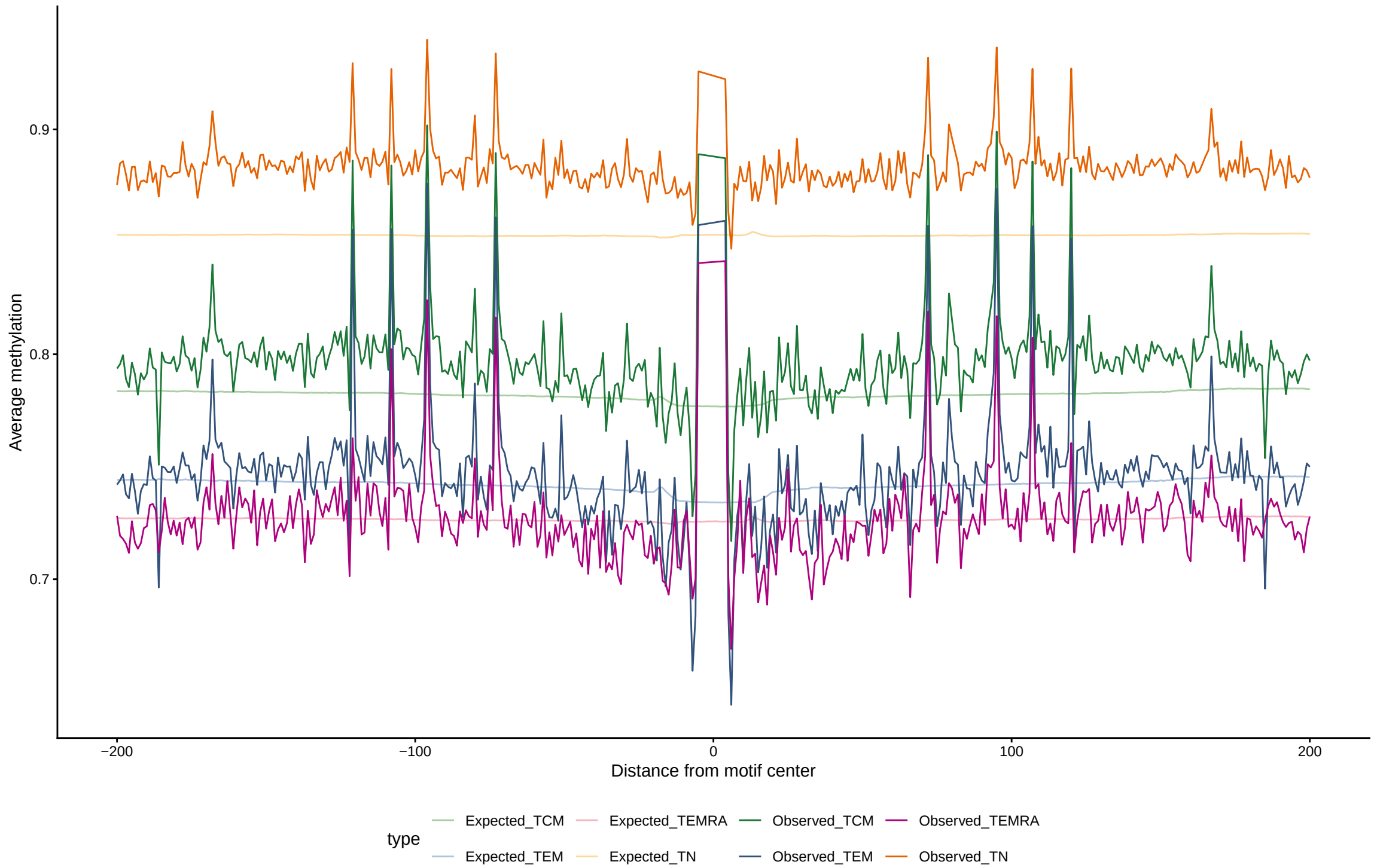
Expected vs observed footprints for HOXA13
