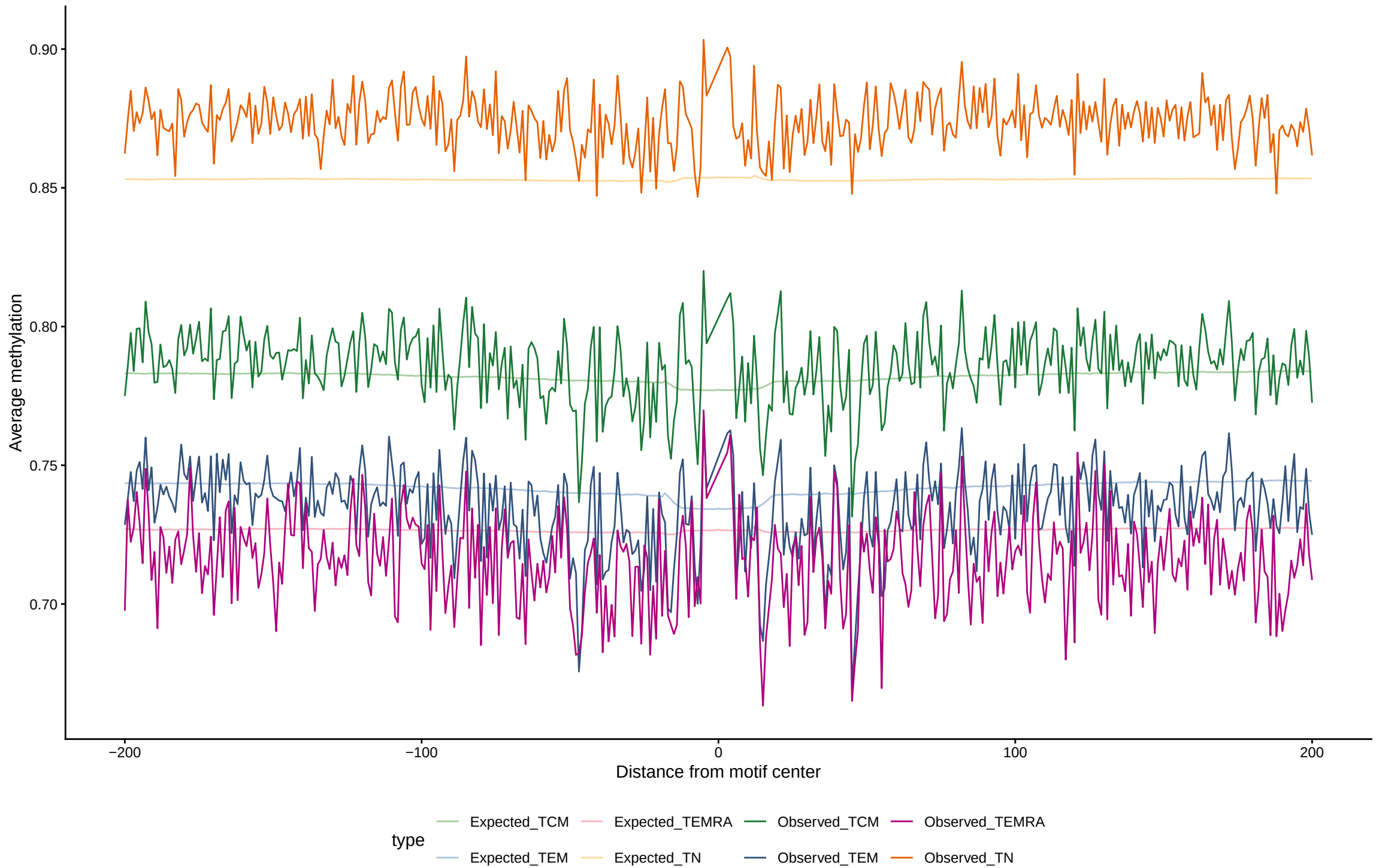
Expected vs observed footprints for HOXB8
