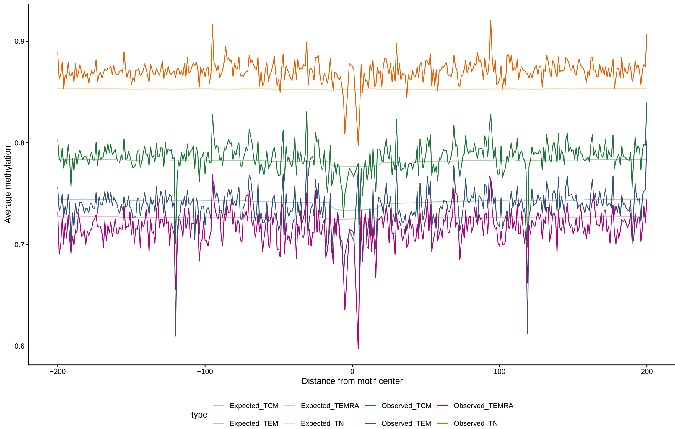
Expected vs observed footprints for HOXC13
