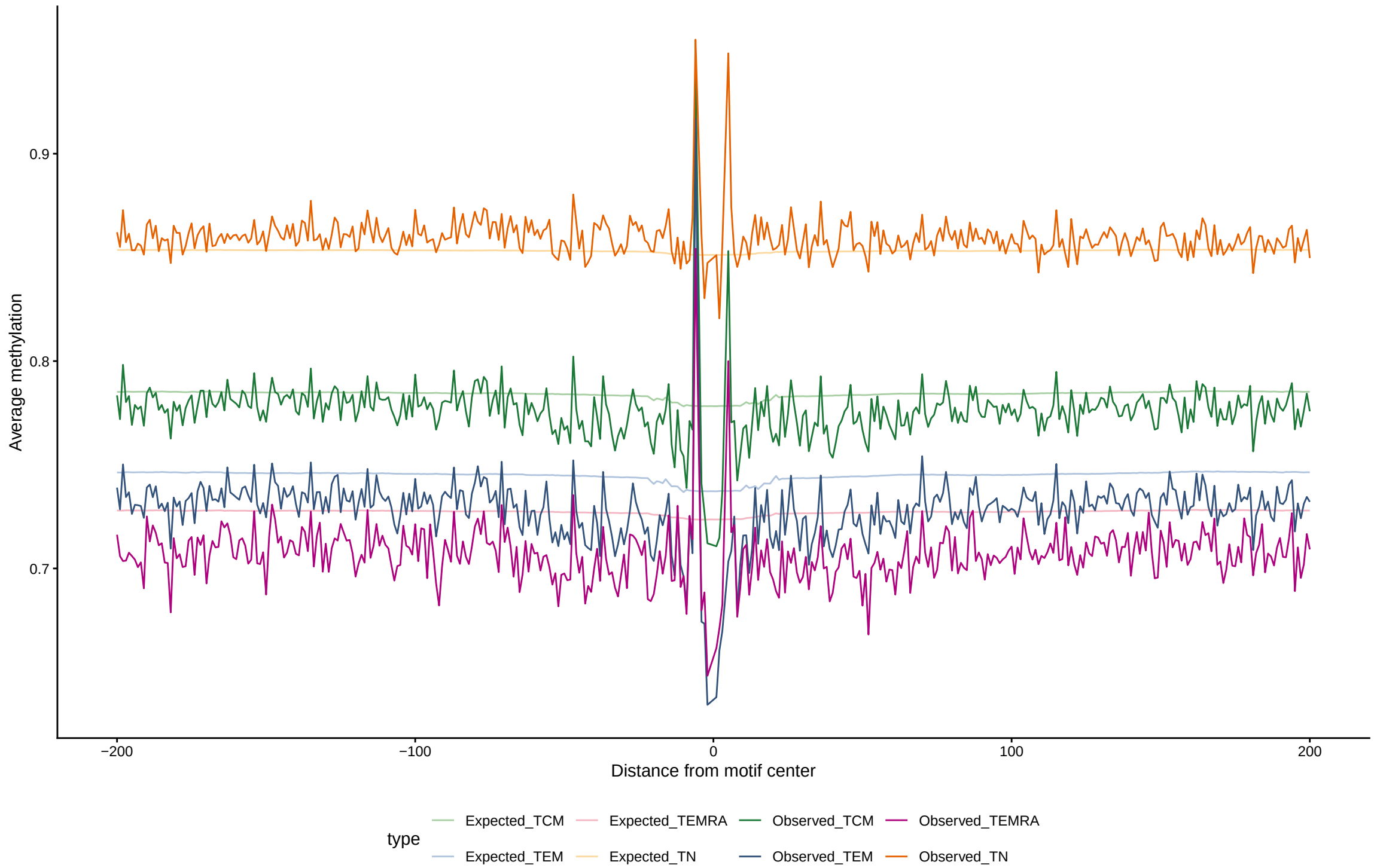
Expected vs observed footprints for HSF1
