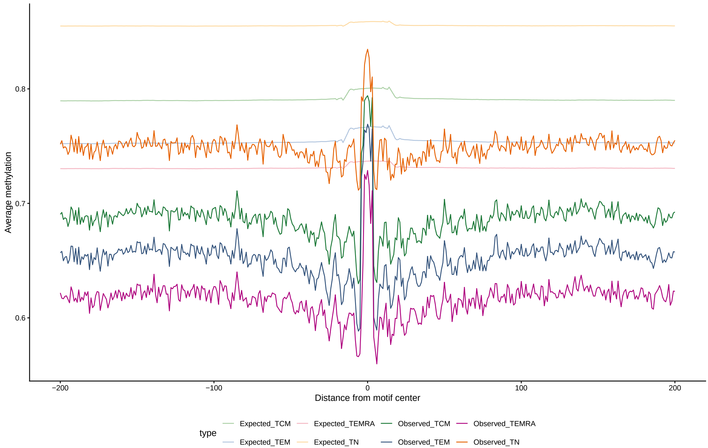
Expected vs observed footprints for INSM1
