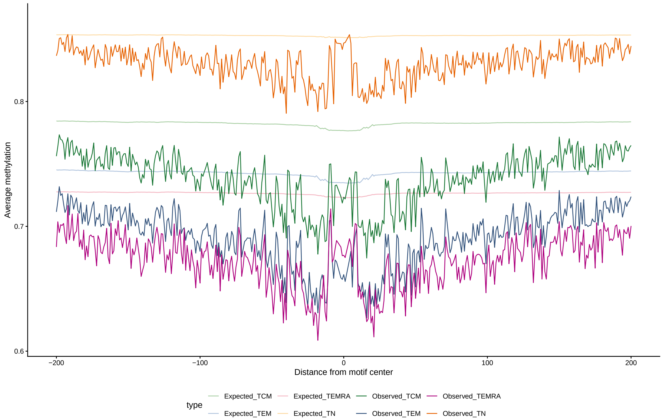
Expected vs observed footprints for IRF8
