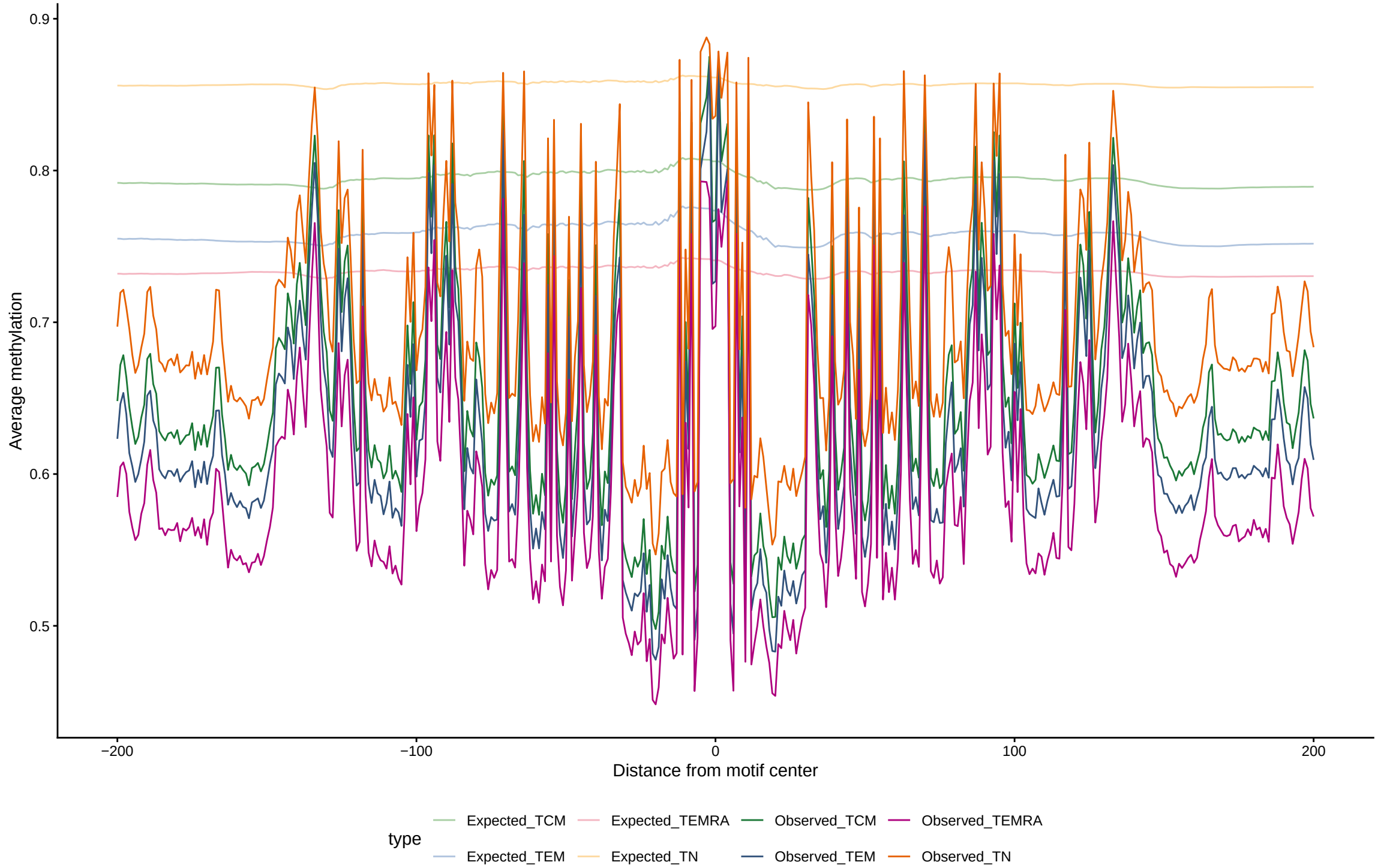
Expected vs observed footprints for KLF2
