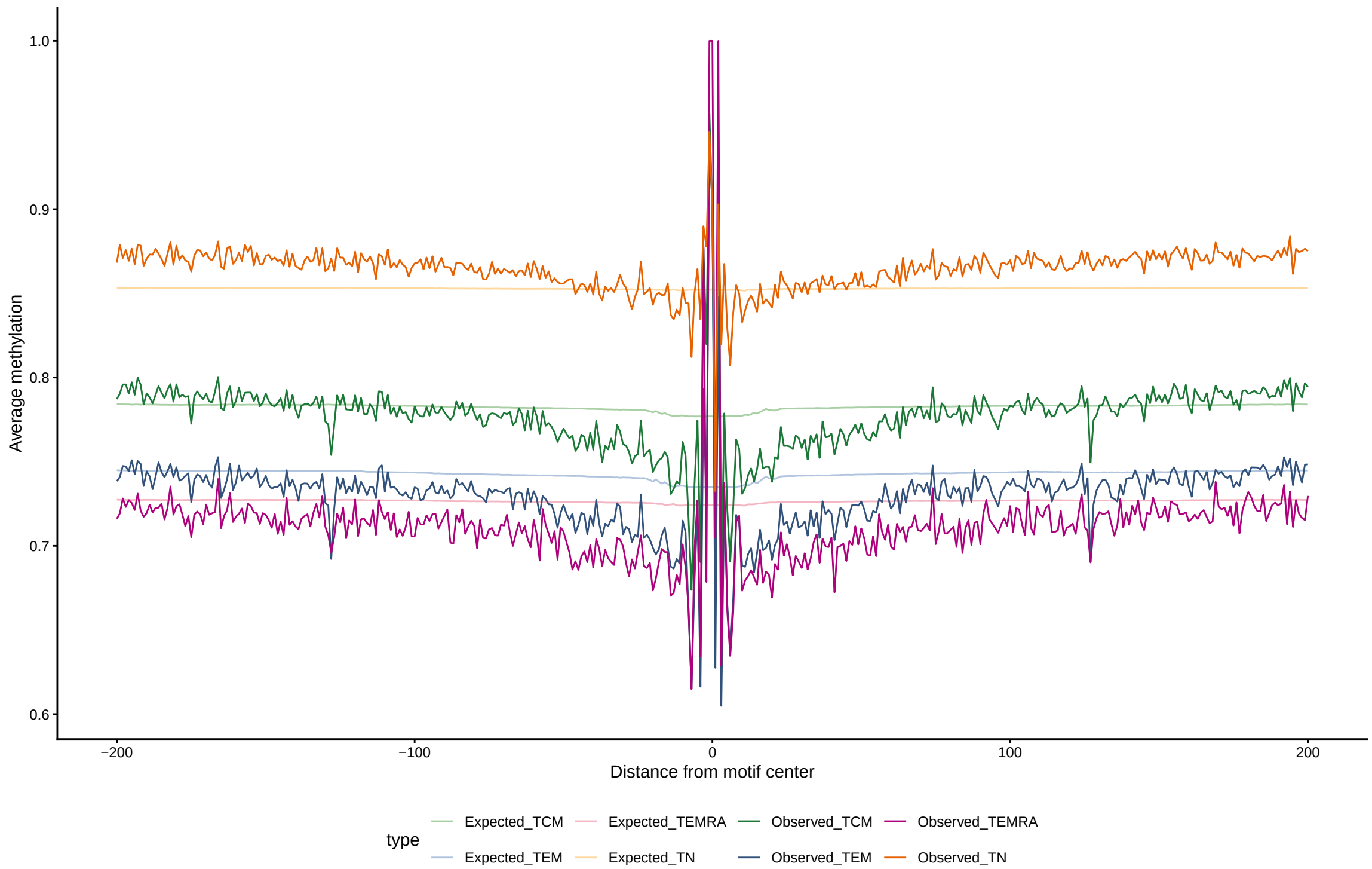
Expected vs observed footprints for LEF1
