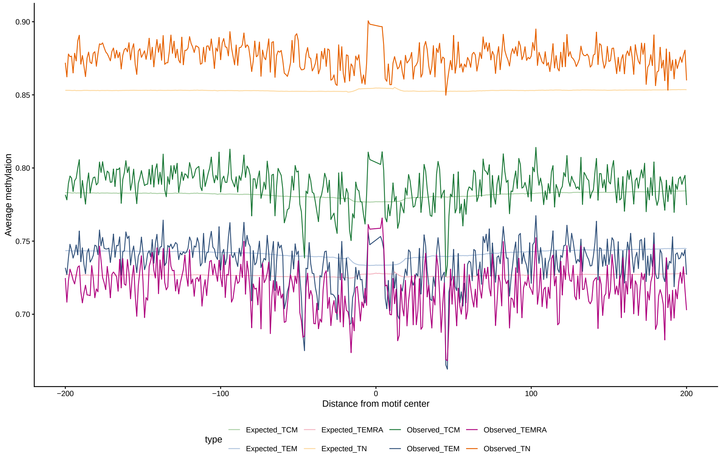
Expected vs observed footprints for LHX5
