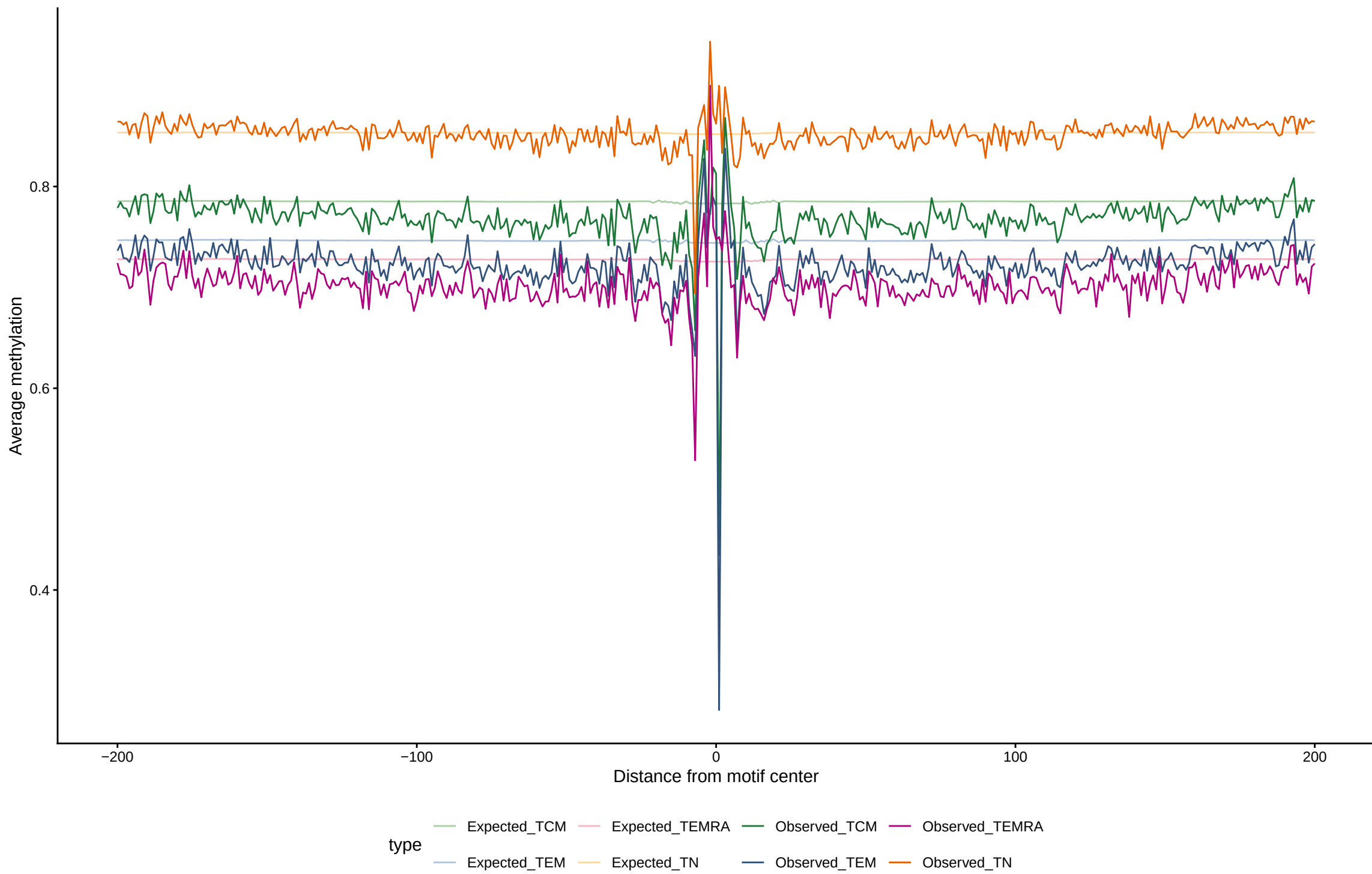
Expected vs observed footprints for MAF
