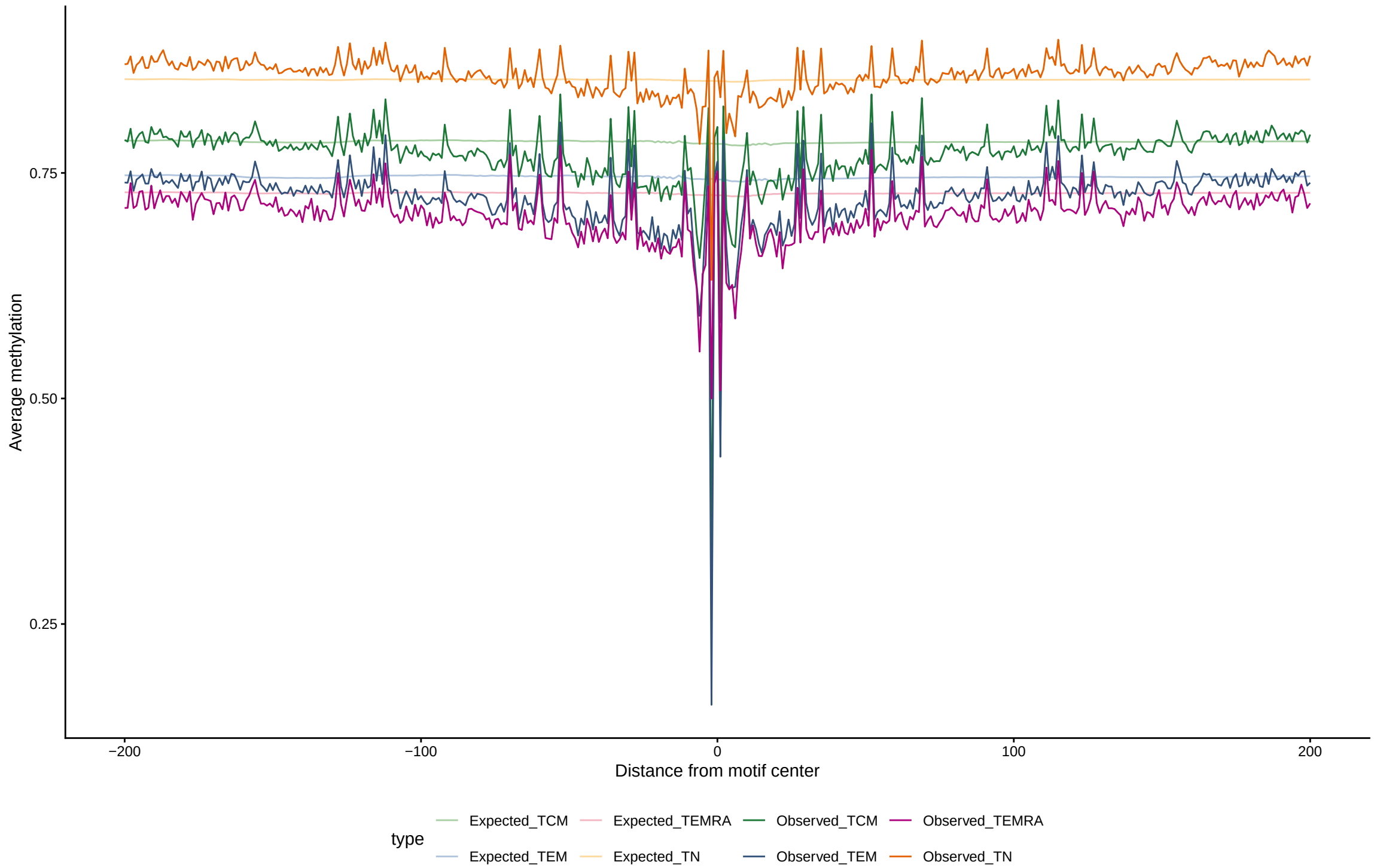
Expected vs observed footprints for MAF::NFE2
